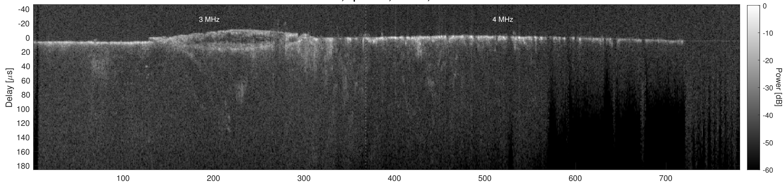
Orbit 9610, Cluttergram
