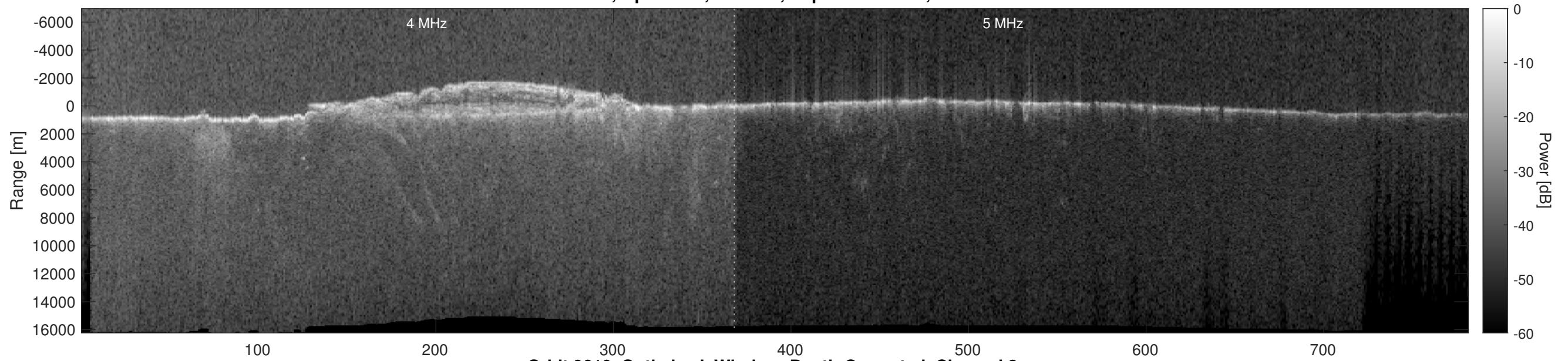
Orbit 9610, Optimized, Window, Depth-Corrected, Channel 2
