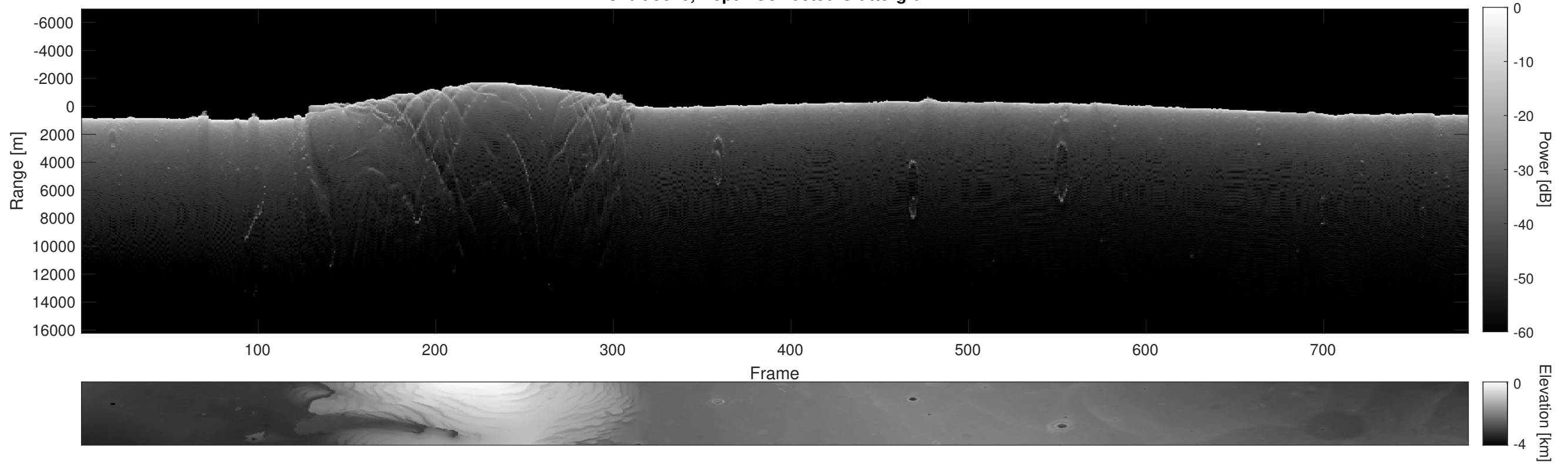
Orbit 9610, Depth-Corrected Cluttergram
