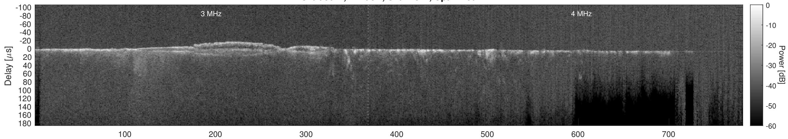
Orbit 9611, Cluttergram
