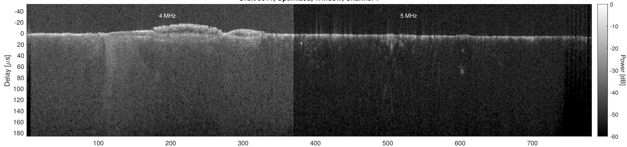
Orbit 9611, Optimized, Window, Channel 2
