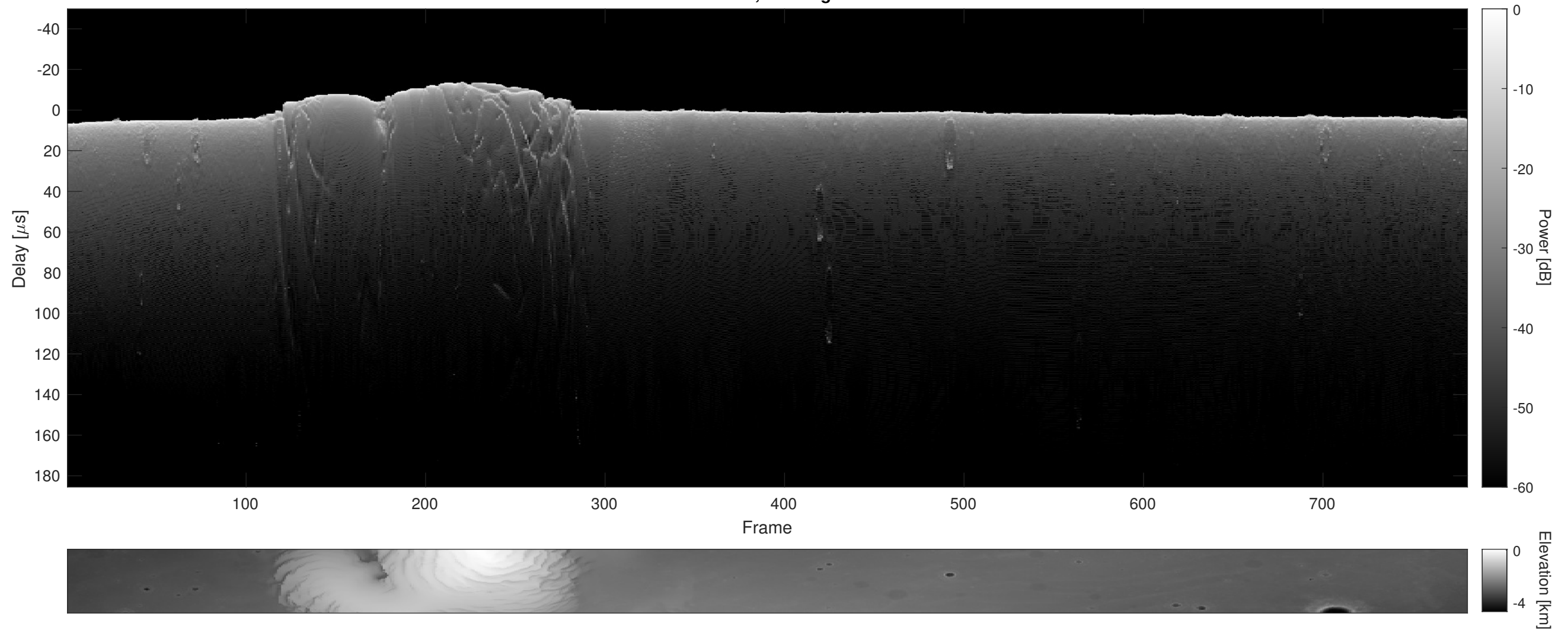
Orbit 9613, Cluttergram
