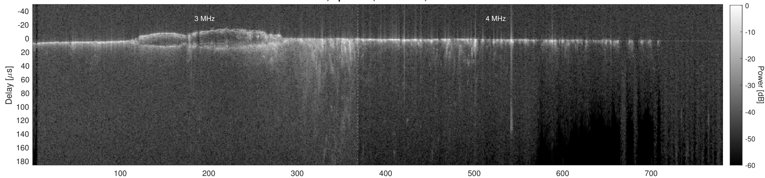
Orbit 9613, Cluttergram
