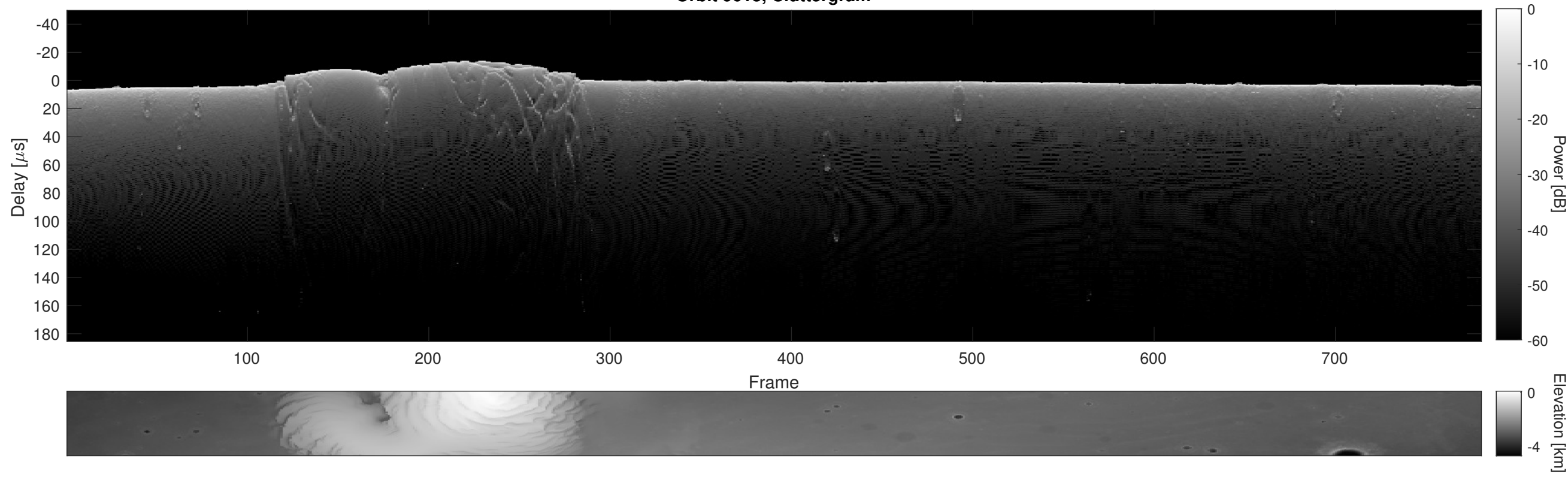
Orbit 9613, Cluttergram
