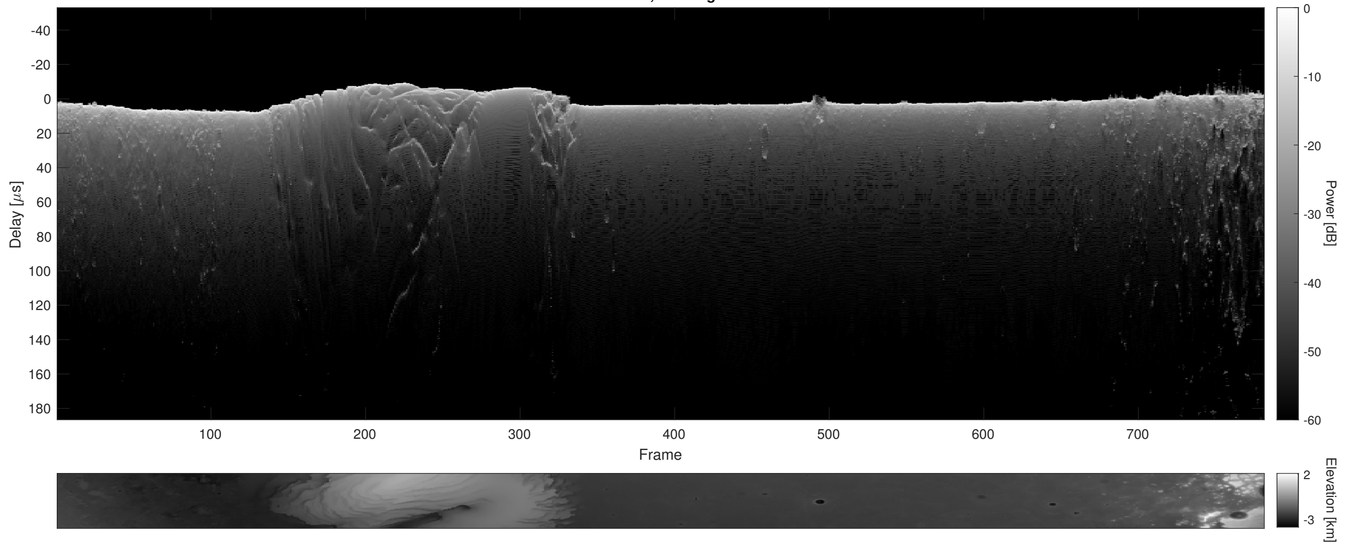
Orbit 9614, Cluttergram
