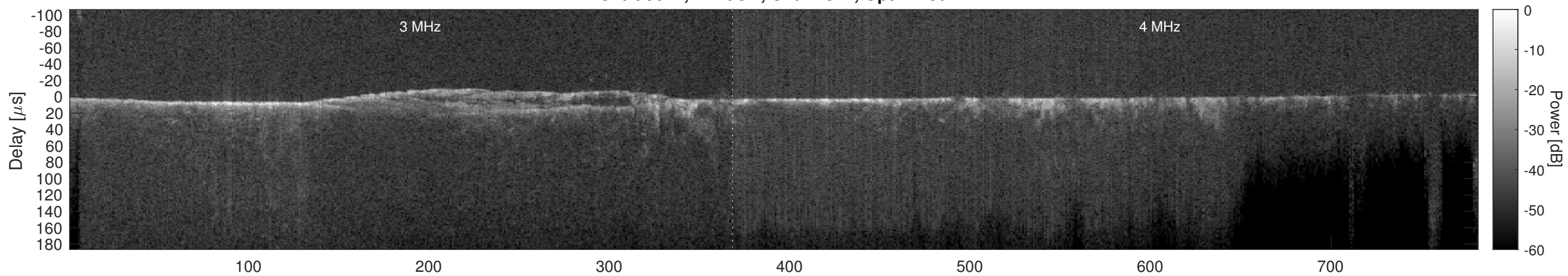
Orbit 9614, Cluttergram
