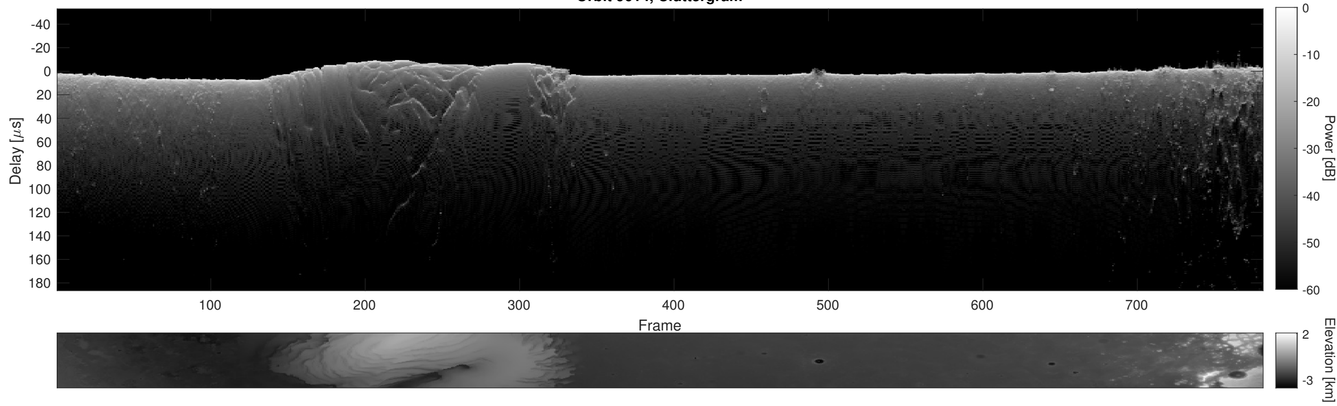
Orbit 9614, Cluttergram
