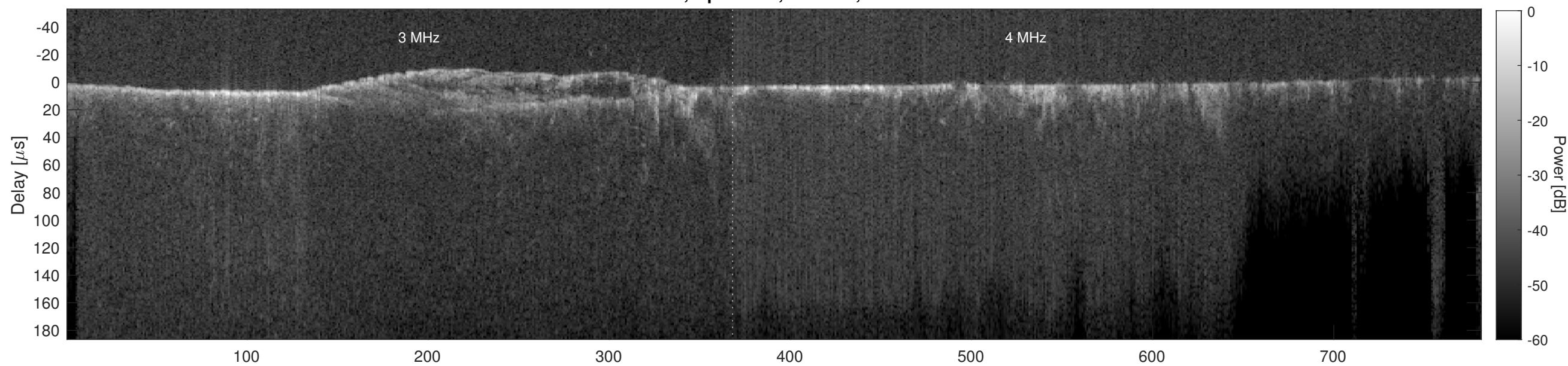
Orbit 9614, Cluttergram
