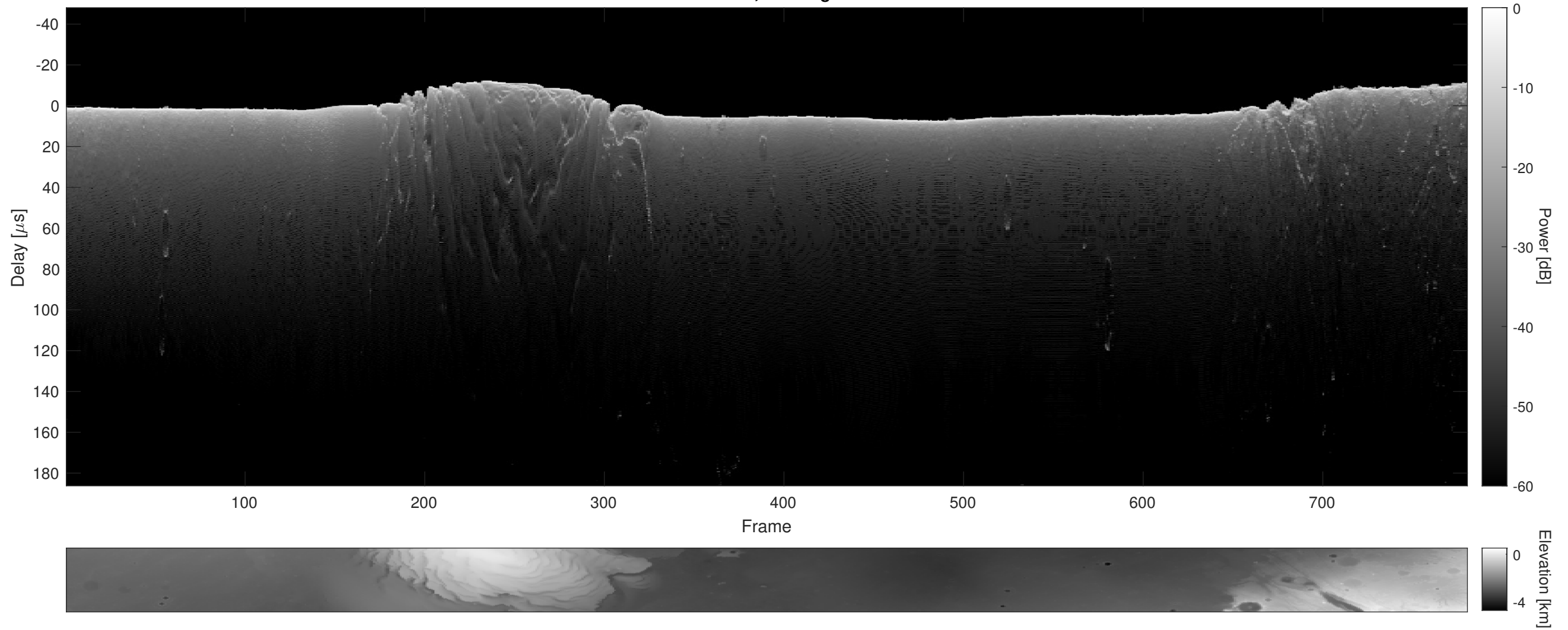
Orbit 9615, Cluttergram
