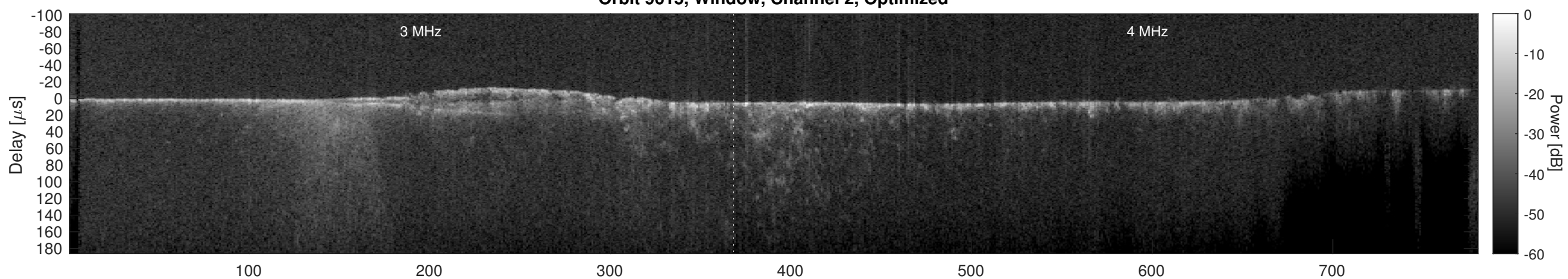
Orbit 9615, Cluttergram
