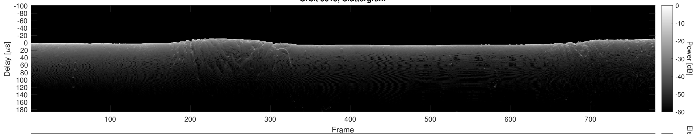
Orbit 9615, Cluttergram
