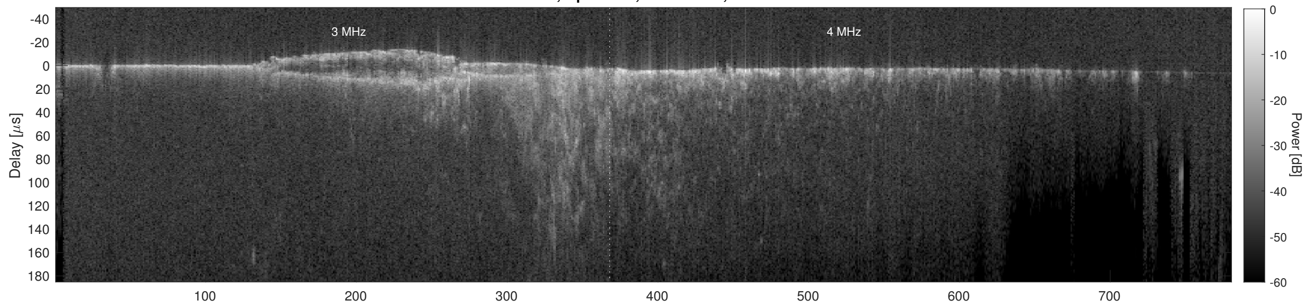
Orbit 9616, Cluttergram
