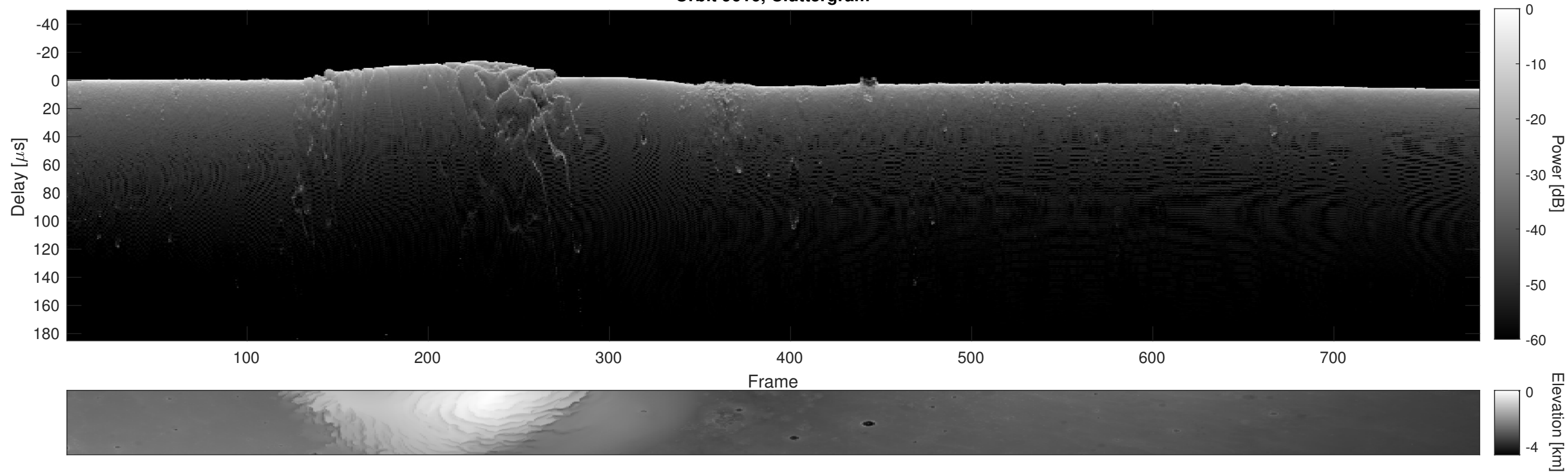
Orbit 9616, Cluttergram
