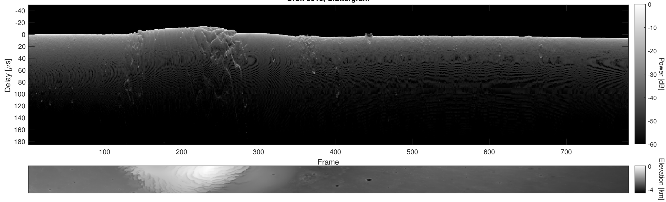
Orbit 9616, Cluttergram
