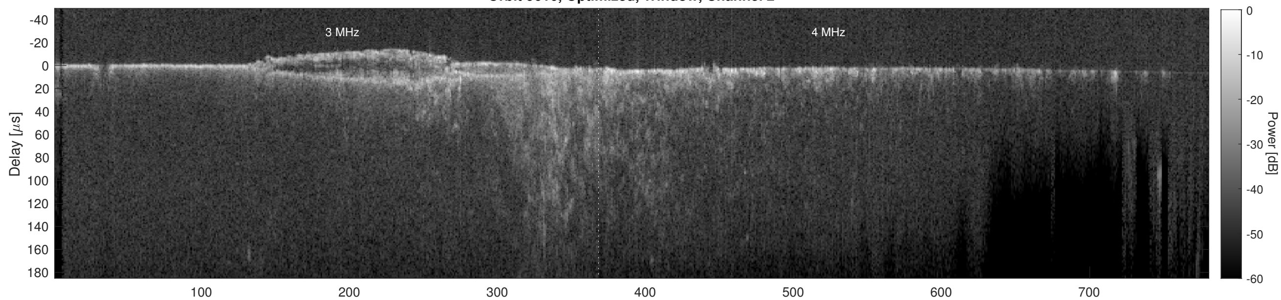
Orbit 9616, Cluttergram
