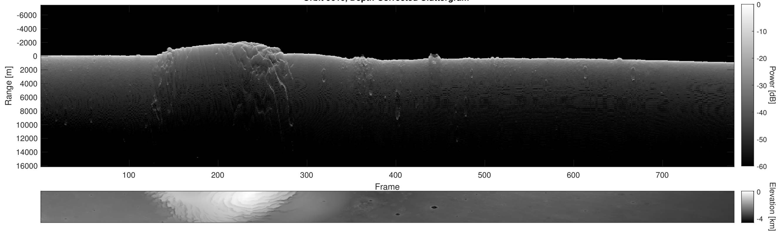
Orbit 9616, Depth-Corrected Cluttergram
