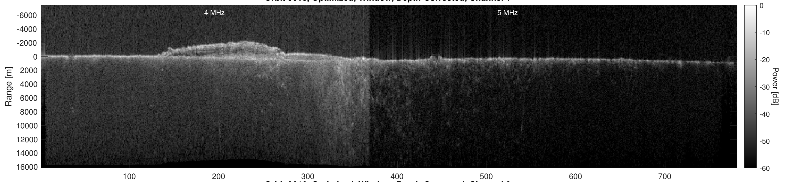
Orbit 9616, Optimized, Window, Depth-Corrected, Channel 2
