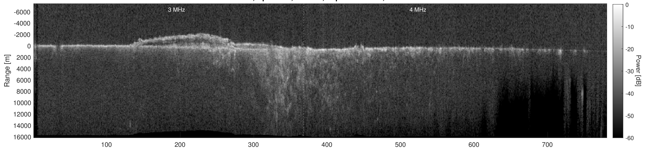
Orbit 9616, Depth-Corrected Cluttergram
