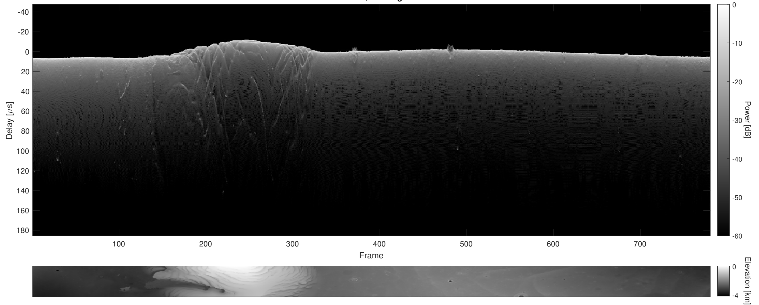
Orbit 9617, Cluttergram
