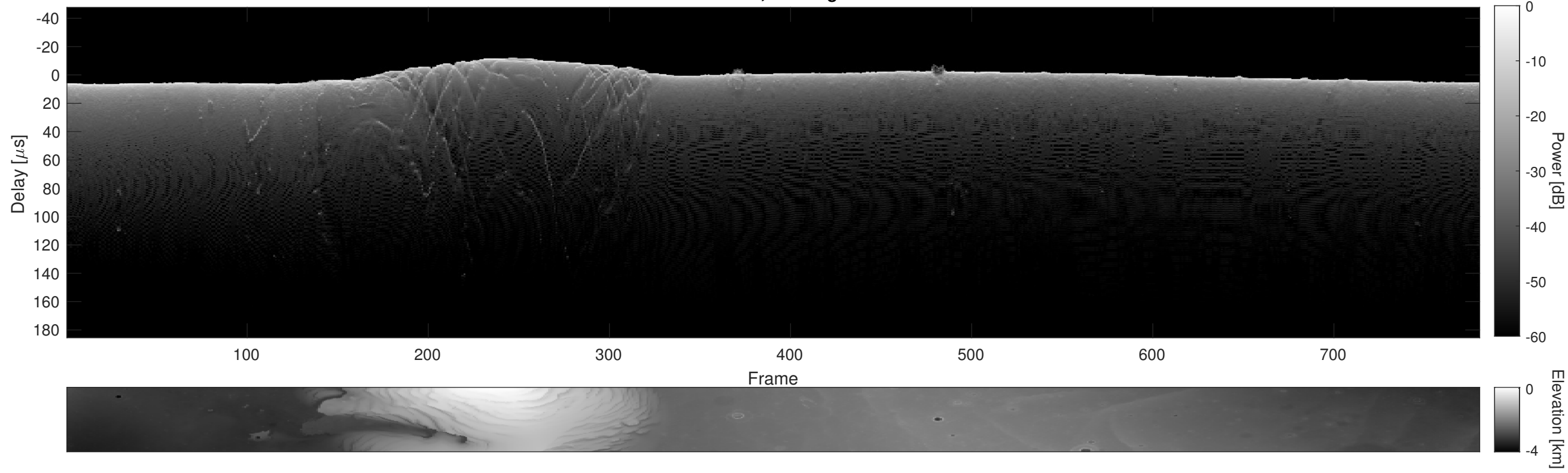
Orbit 9617, Cluttergram
