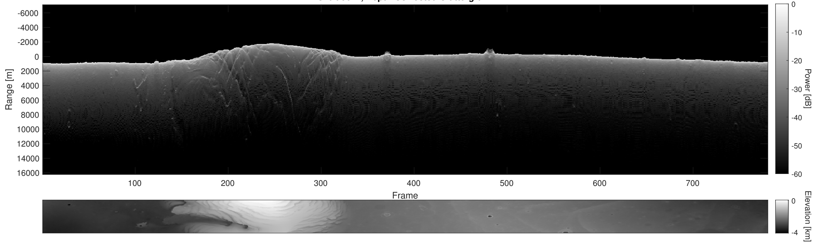
Orbit 9617, Depth-Corrected Cluttergram
