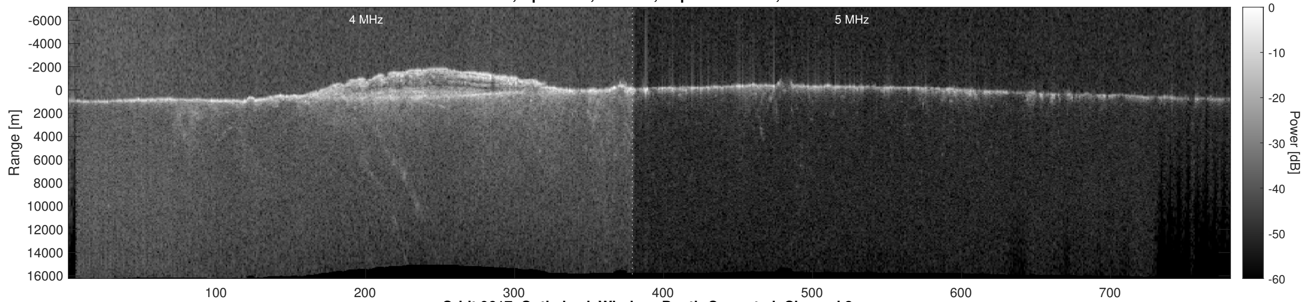
Orbit 9617, Optimized, Window, Depth-Corrected, Channel 2
