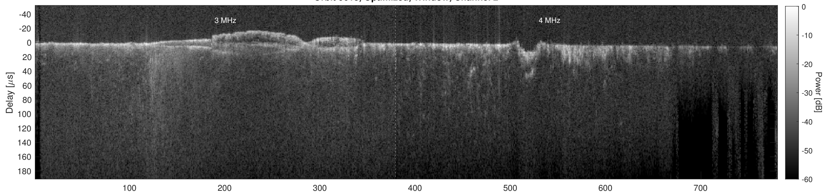
Orbit 9618, Cluttergram
