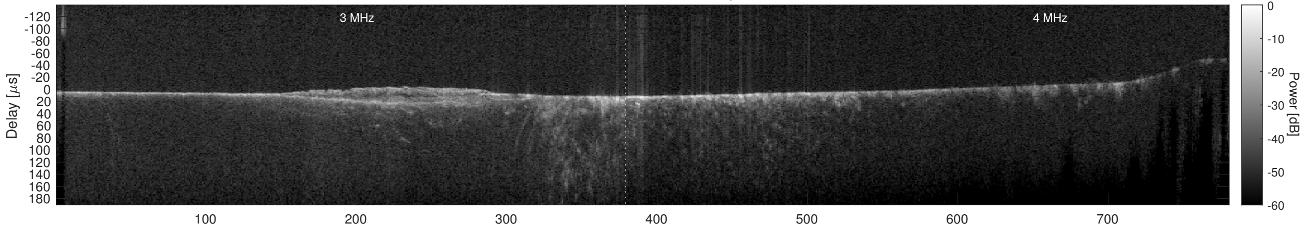
Orbit 9619, Cluttergram
