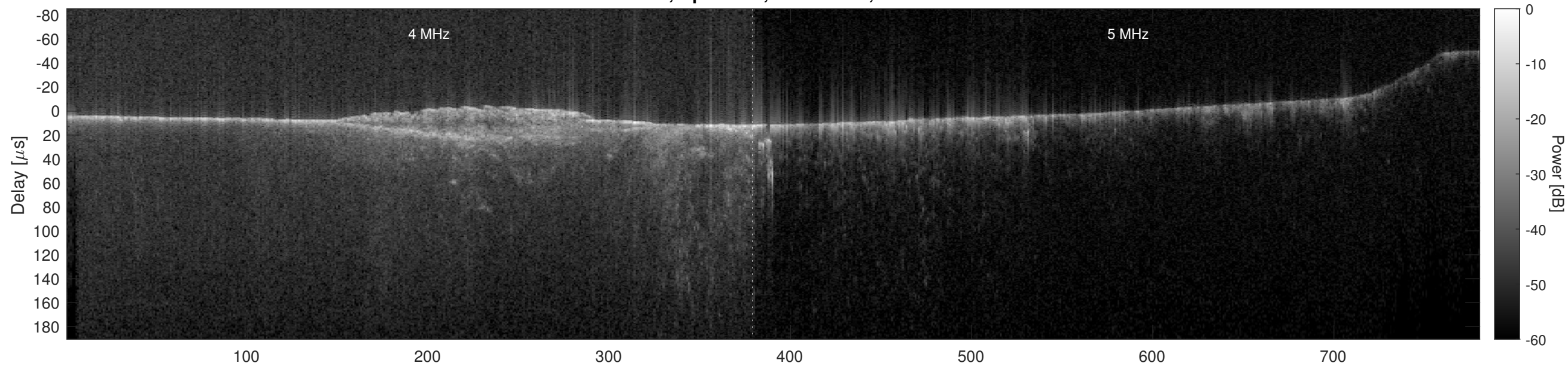
Orbit 9619, Optimized, No Window, Channel 2
