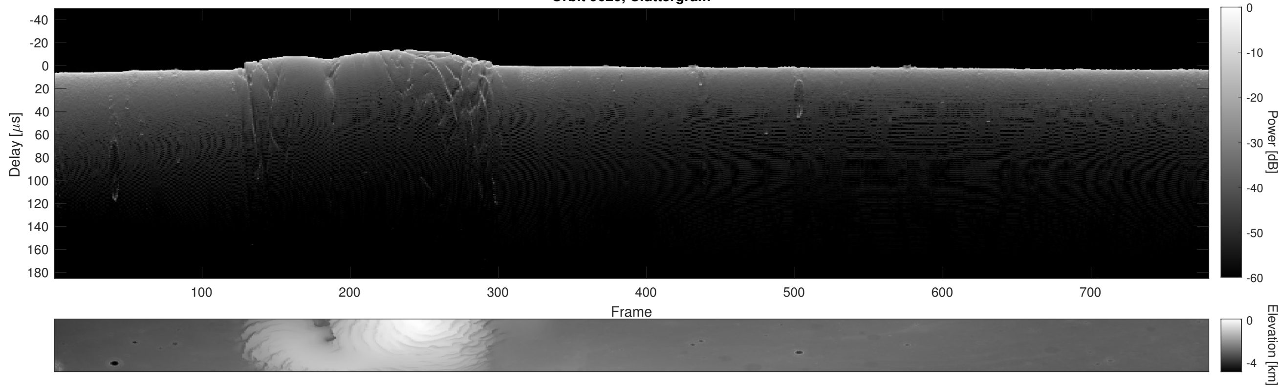
Orbit 9620, Cluttergram
