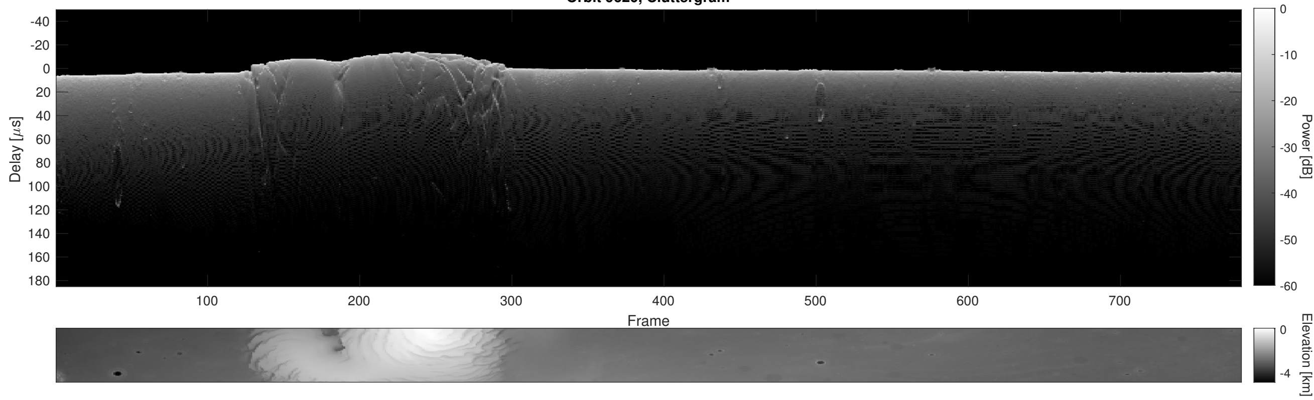
Orbit 9620, Cluttergram
