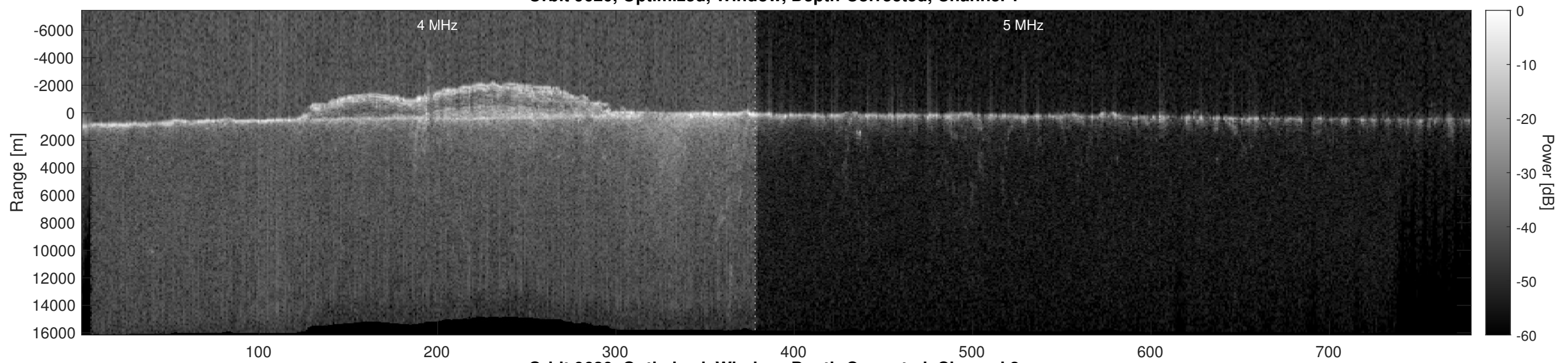
Orbit 9620, Optimized, Window, Depth-Corrected, Channel 2
