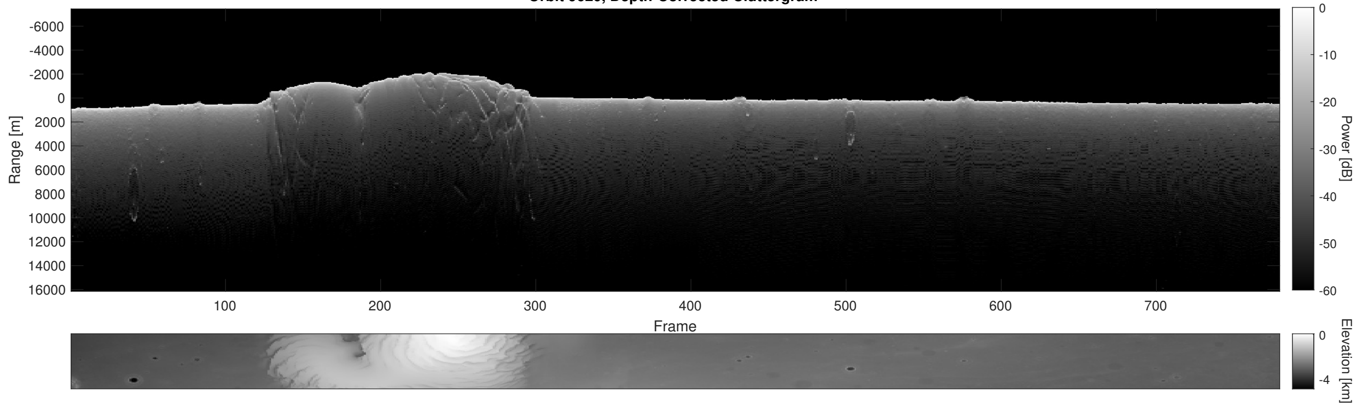
Orbit 9620, Depth-Corrected Cluttergram
