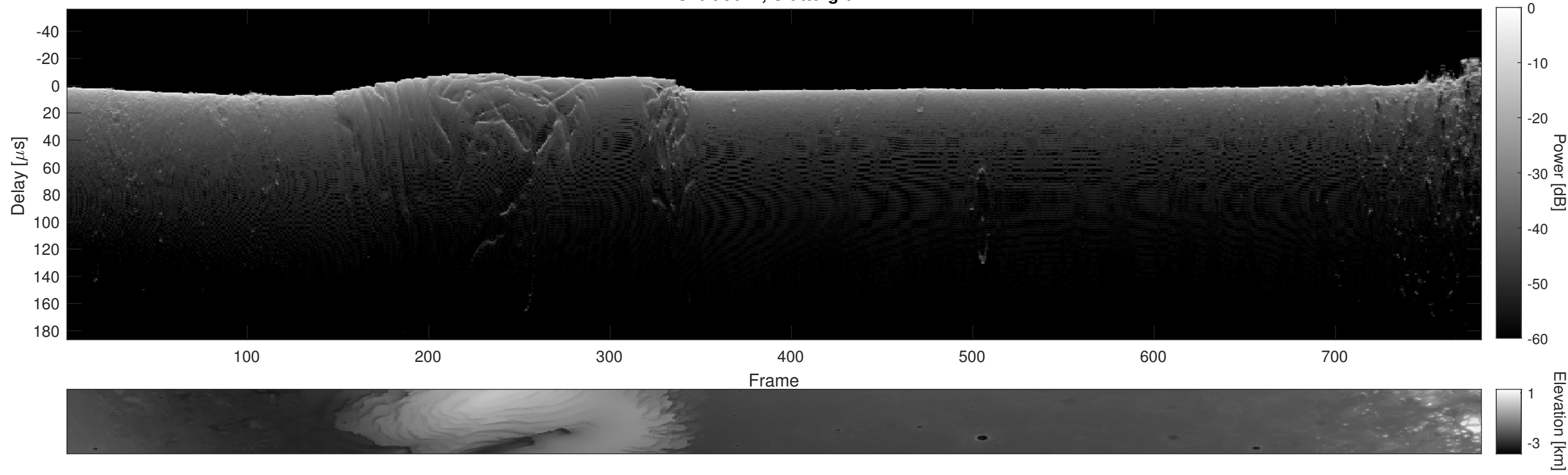
Orbit 9621, Cluttergram
