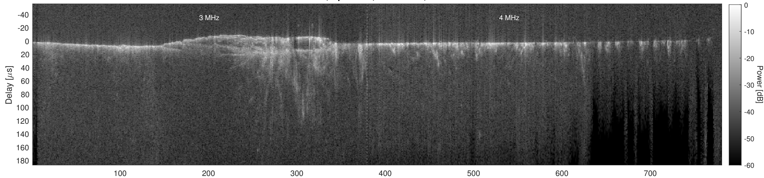
Orbit 9621, Cluttergram
