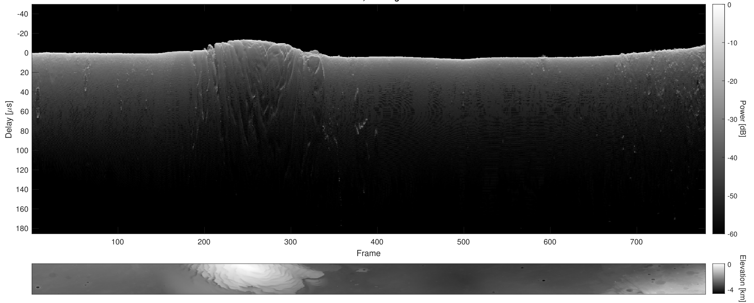
Orbit 9622, Cluttergram
