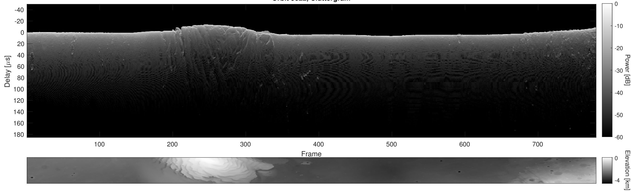
Orbit 9622, Cluttergram
