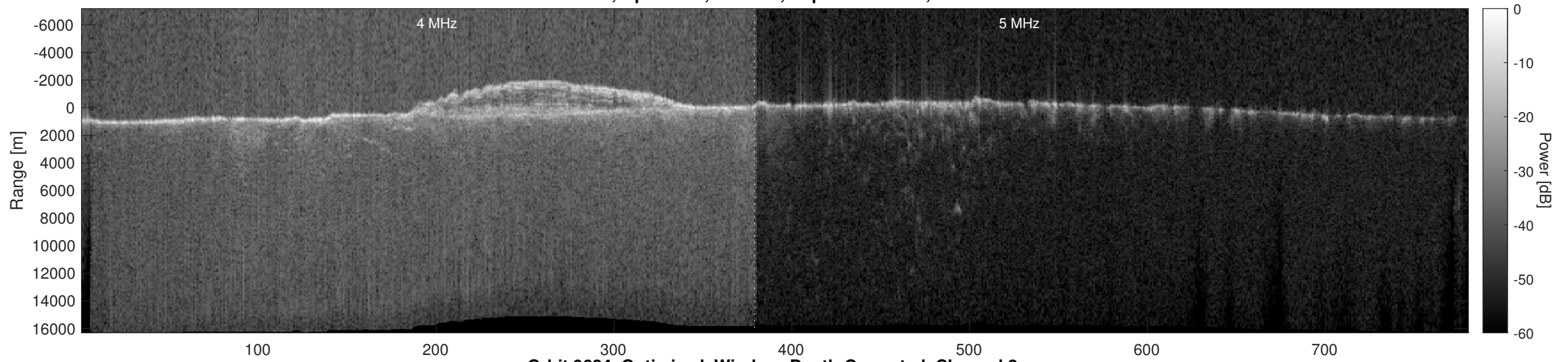
Orbit 9624, Optimized, Window, Depth-Corrected, Channel 2
