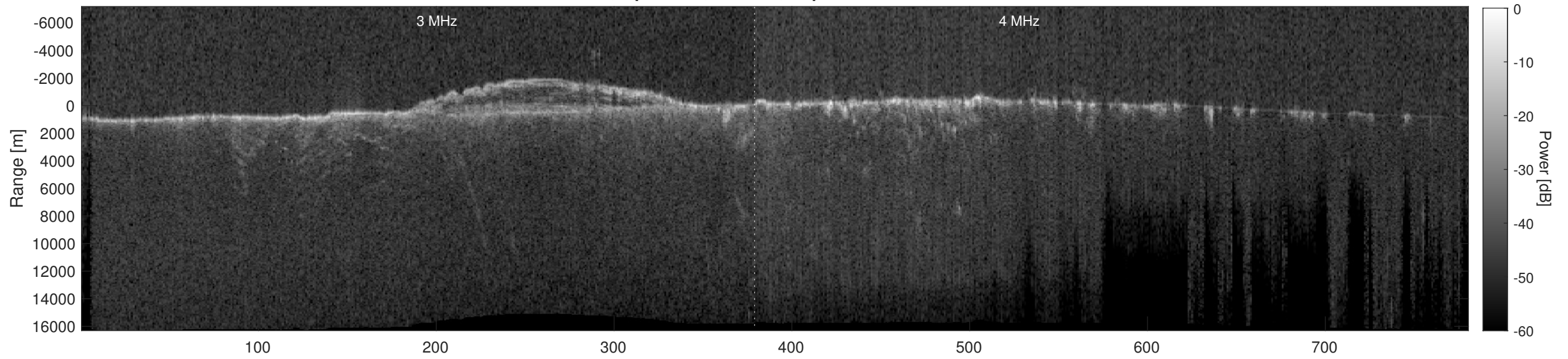
Orbit 9624, Depth-Corrected Cluttergram
