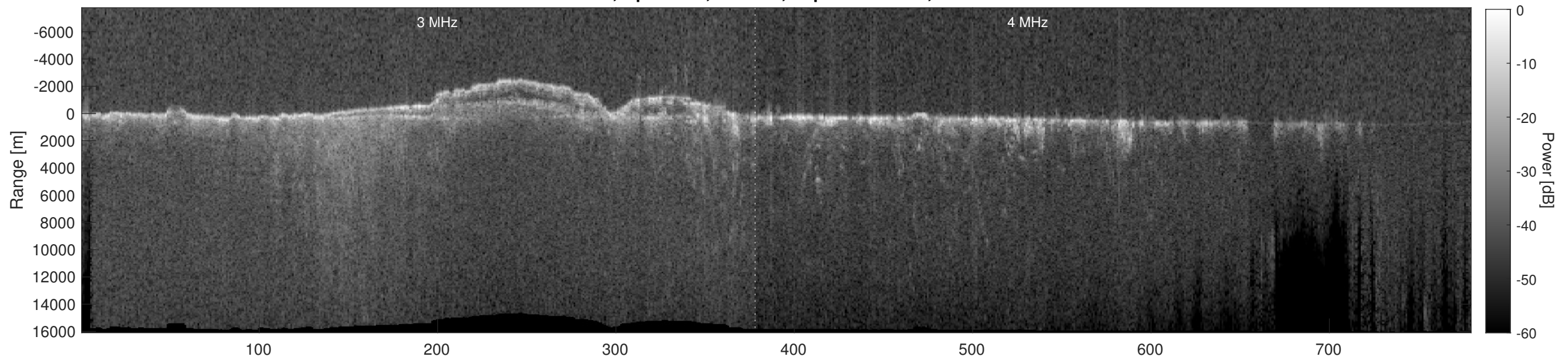
Orbit 9625, Depth-Corrected Cluttergram
