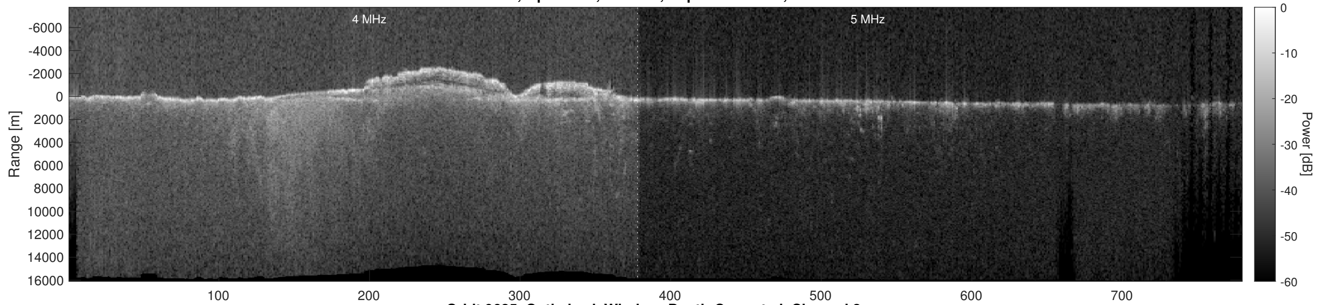
Orbit 9625, Optimized, Window, Depth-Corrected, Channel 2
