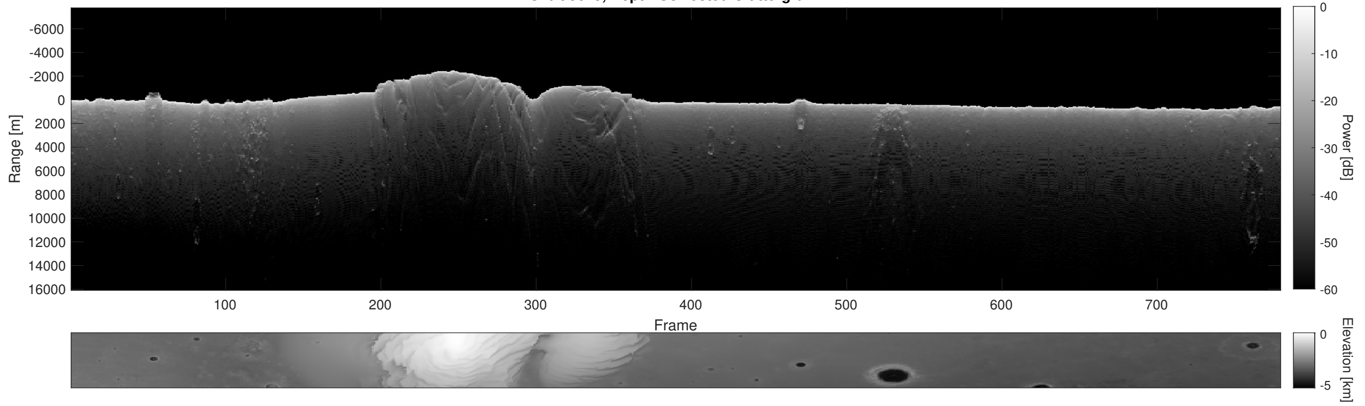
Orbit 9625, Depth-Corrected Cluttergram
