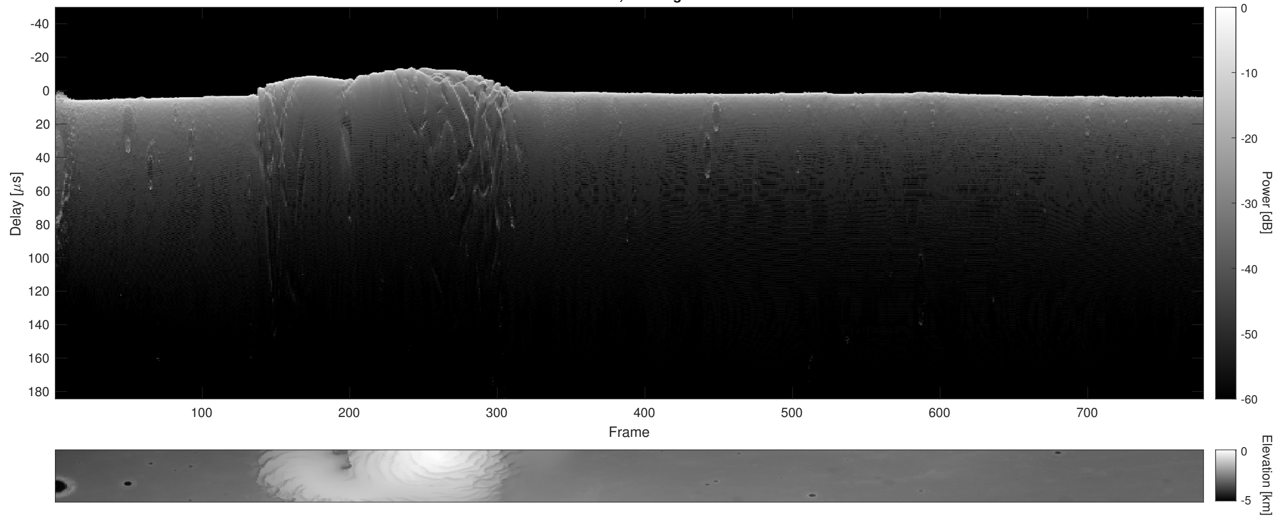
Orbit 9627, Cluttergram
