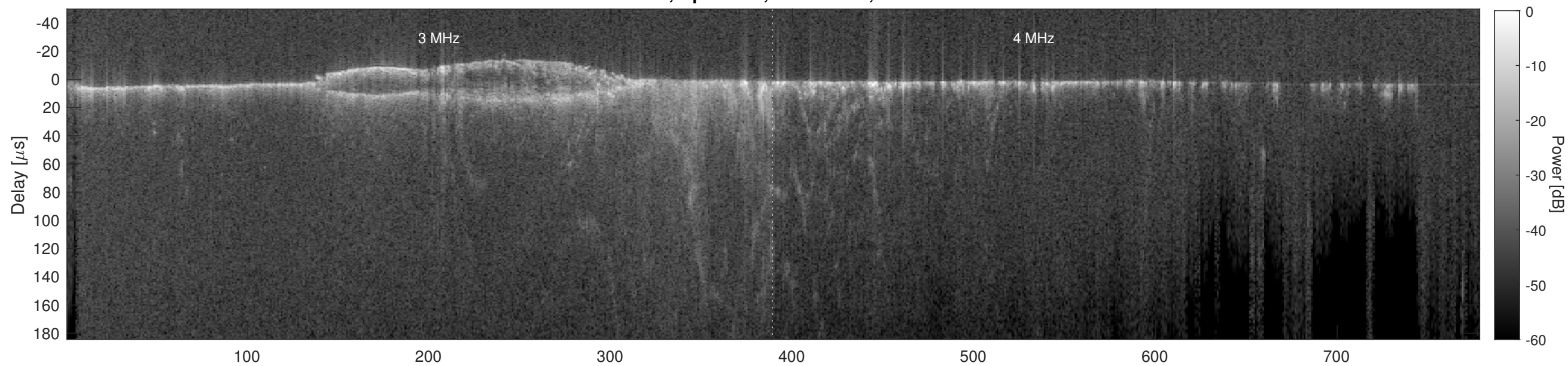
Orbit 9627, Cluttergram
