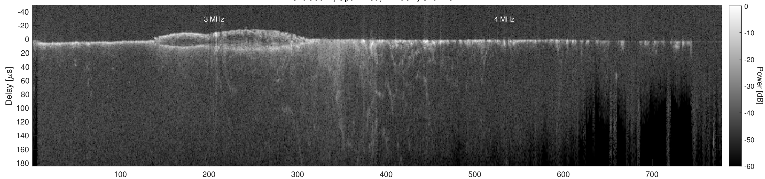
Orbit 9627, Cluttergram
