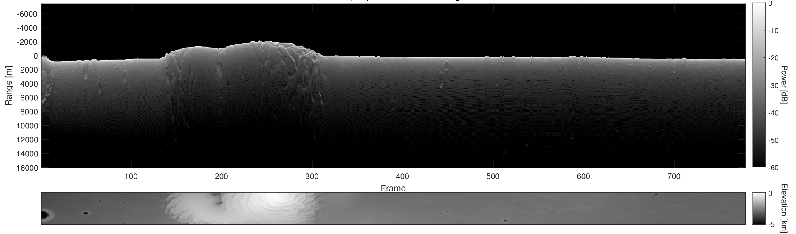
Orbit 9627, Depth-Corrected Cluttergram
