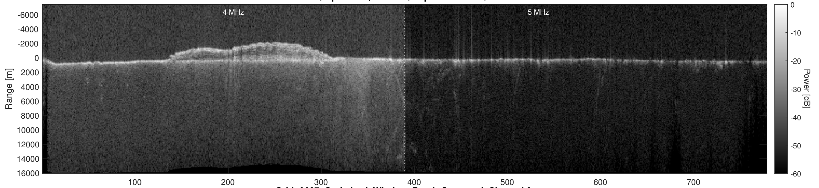
Orbit 9627, Optimized, Window, Depth-Corrected, Channel 2
