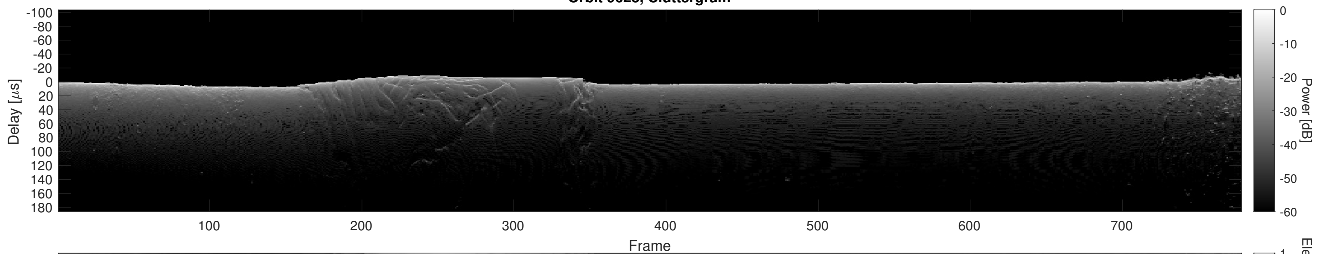
Orbit 9628, Cluttergram
