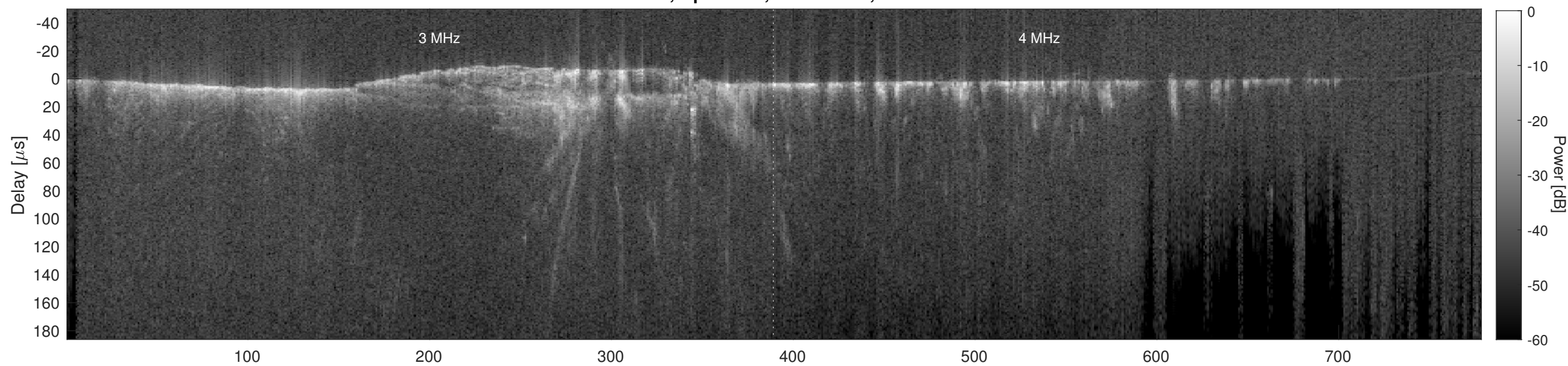
Orbit 9628, Cluttergram
