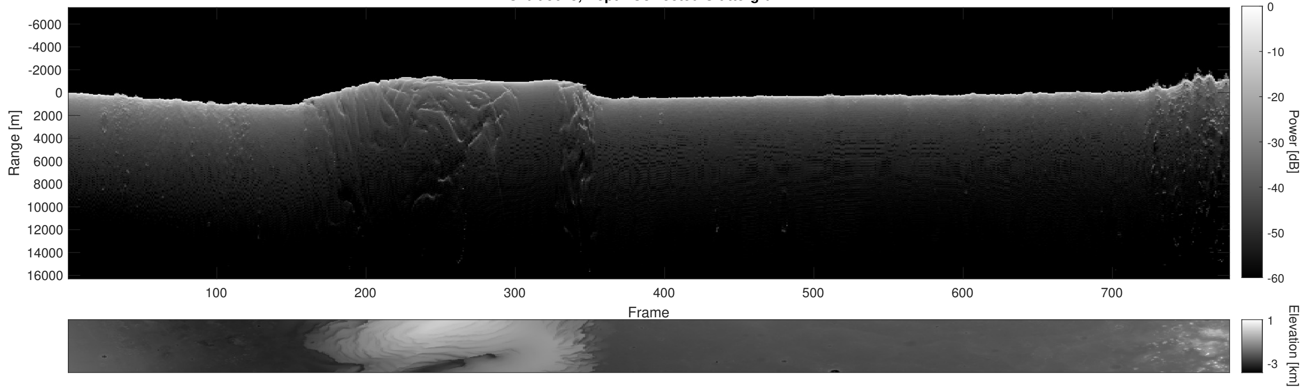
Orbit 9628, Depth-Corrected Cluttergram
