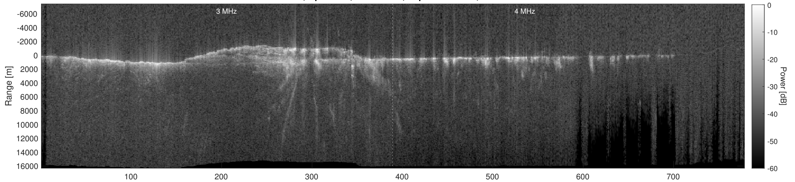
Orbit 9628, Depth-Corrected Cluttergram
