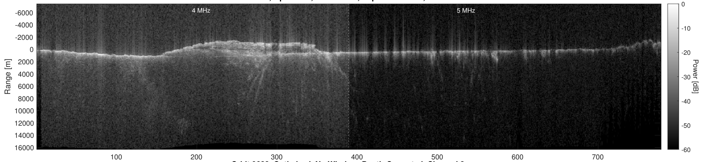
Orbit 9628, Optimized, No Window, Depth-Corrected, Channel 2
