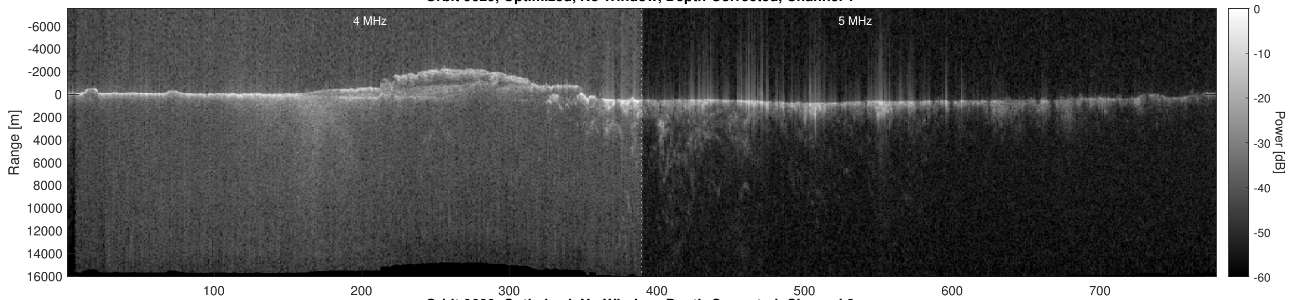
Orbit 9629, Optimized, No Window, Depth-Corrected, Channel 2
