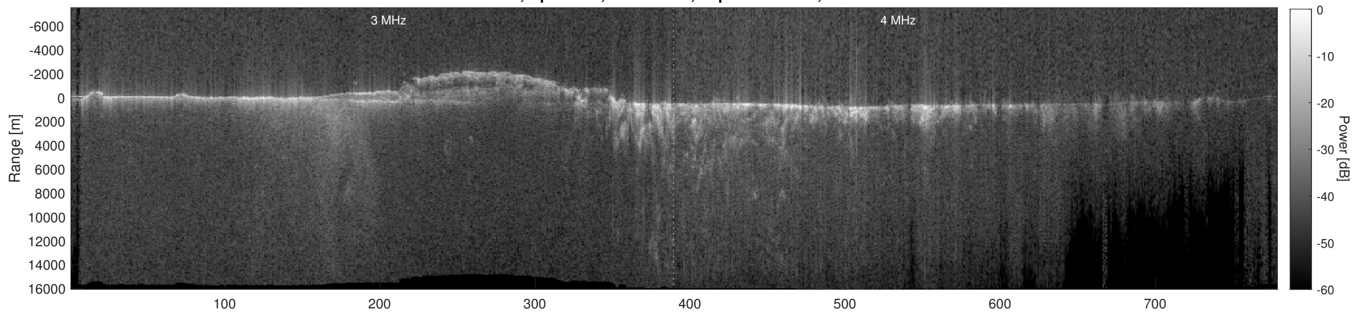
Orbit 9629, Depth-Corrected Cluttergram
