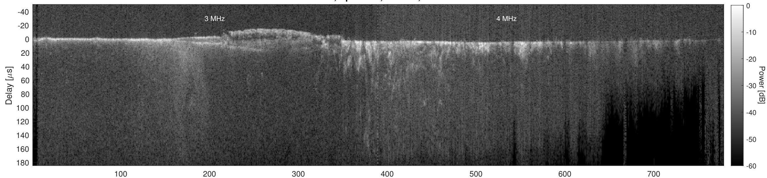
Orbit 9629, Cluttergram
