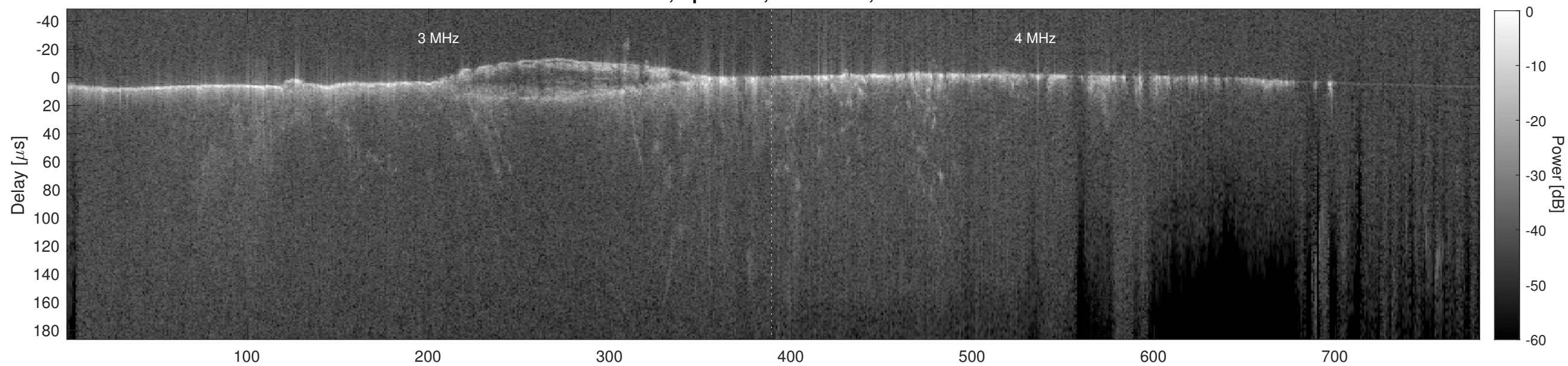
Orbit 9631, Cluttergram
