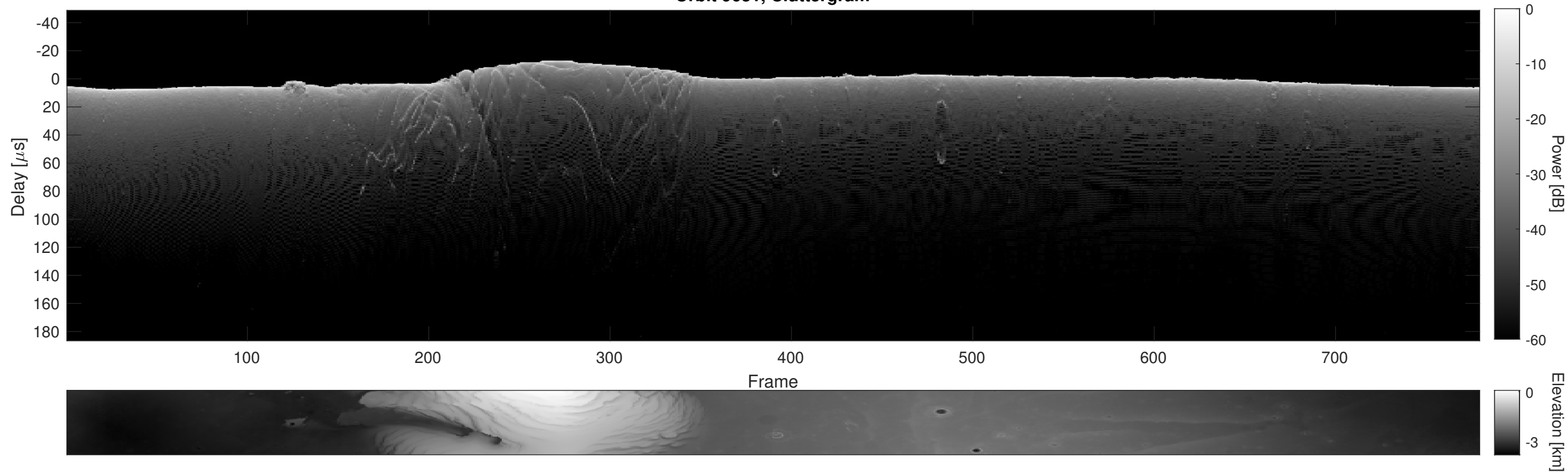
Orbit 9631, Cluttergram
