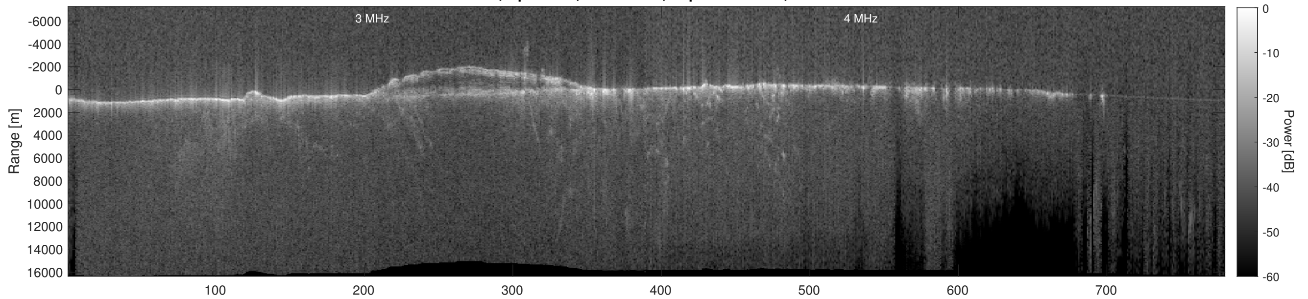
Orbit 9631, Depth-Corrected Cluttergram
