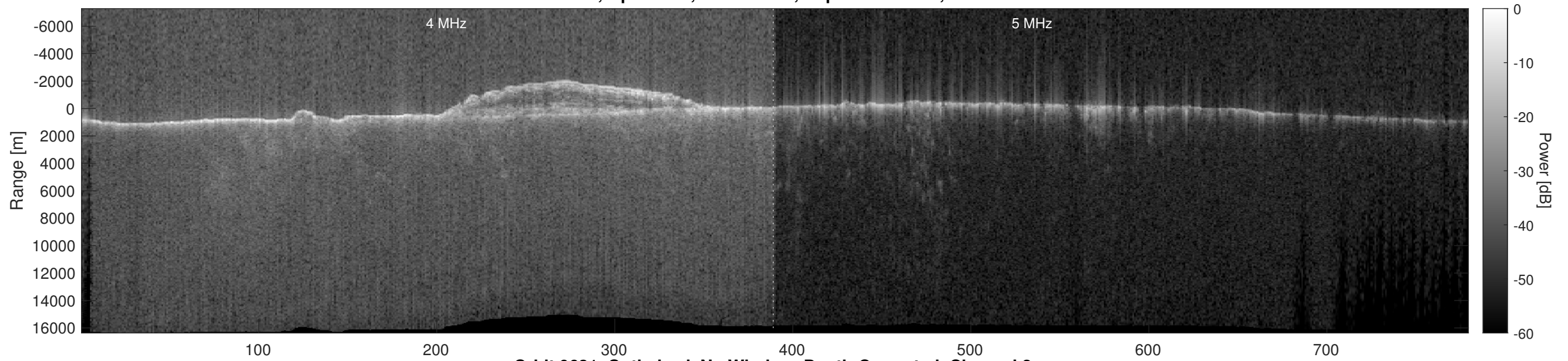
Orbit 9631, Optimized, No Window, Depth-Corrected, Channel 2
