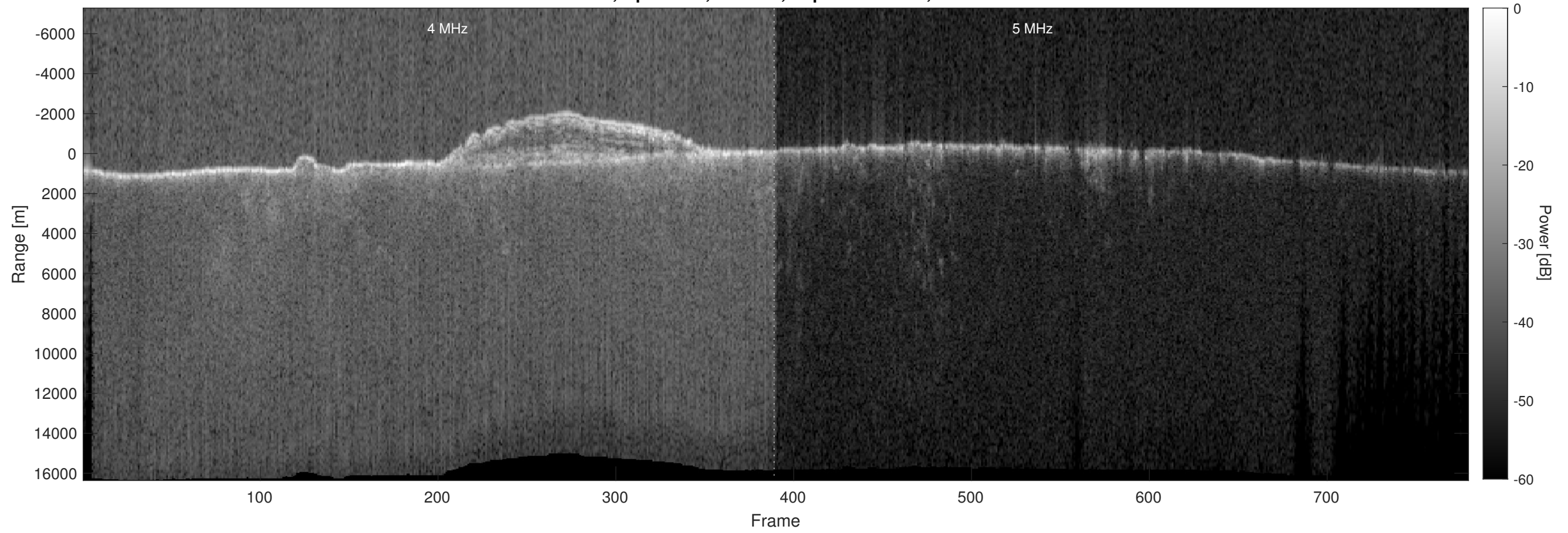
Orbit 9631, Optimized, Window, Depth-Corrected, Channel 2
