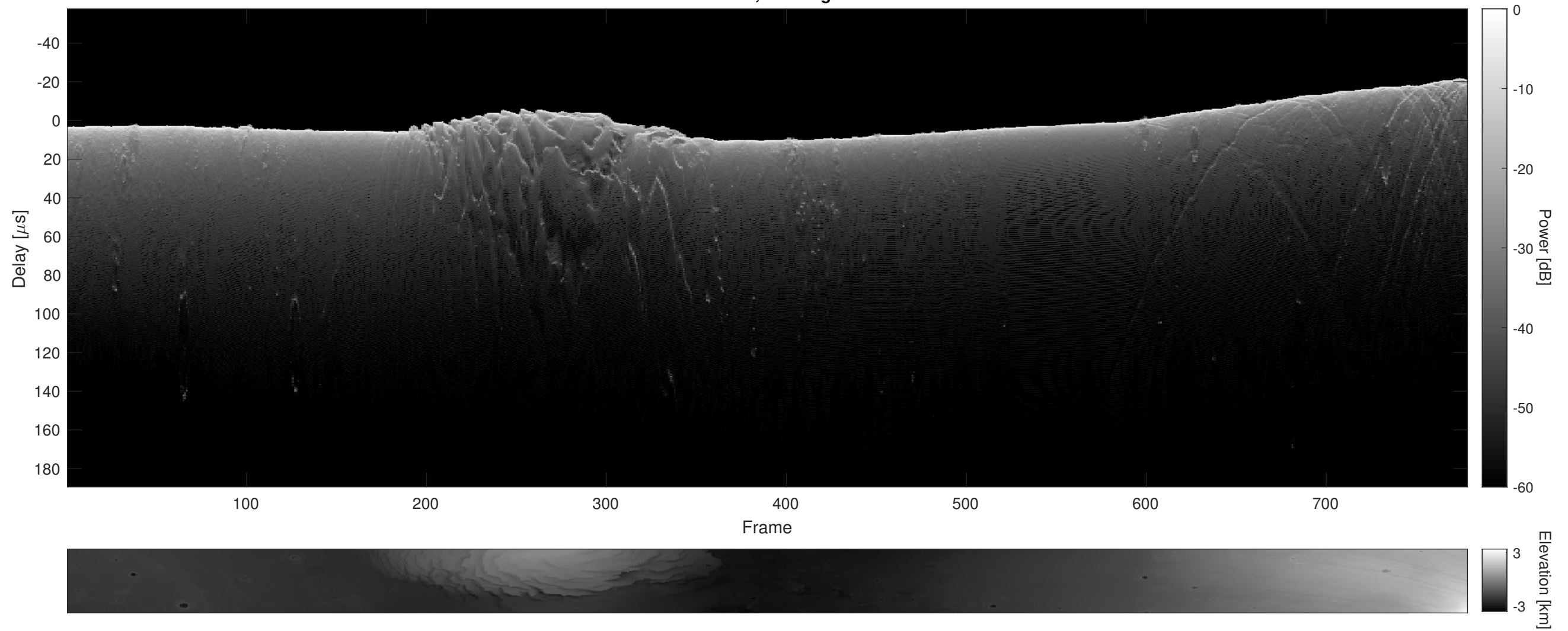
Orbit 9633, Cluttergram
