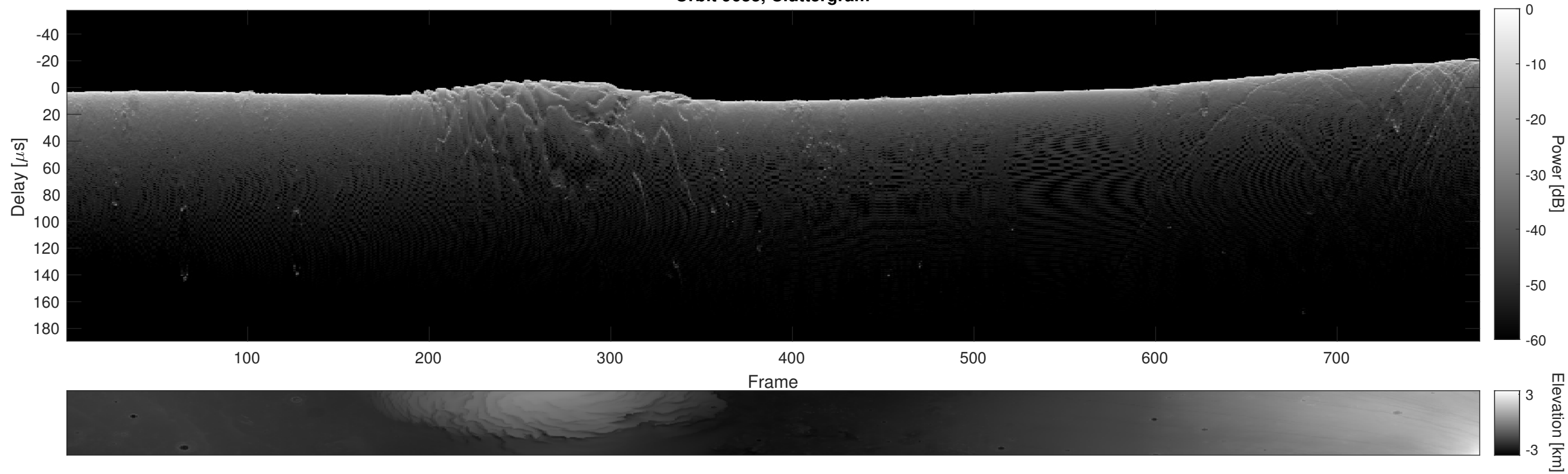
Orbit 9633, Cluttergram
