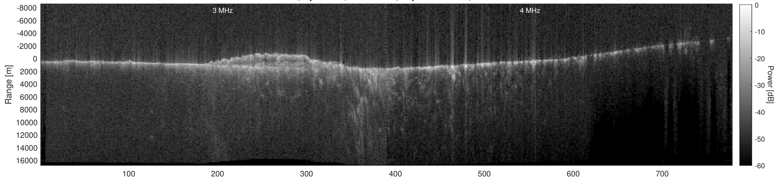
Orbit 9633, Depth-Corrected Cluttergram
