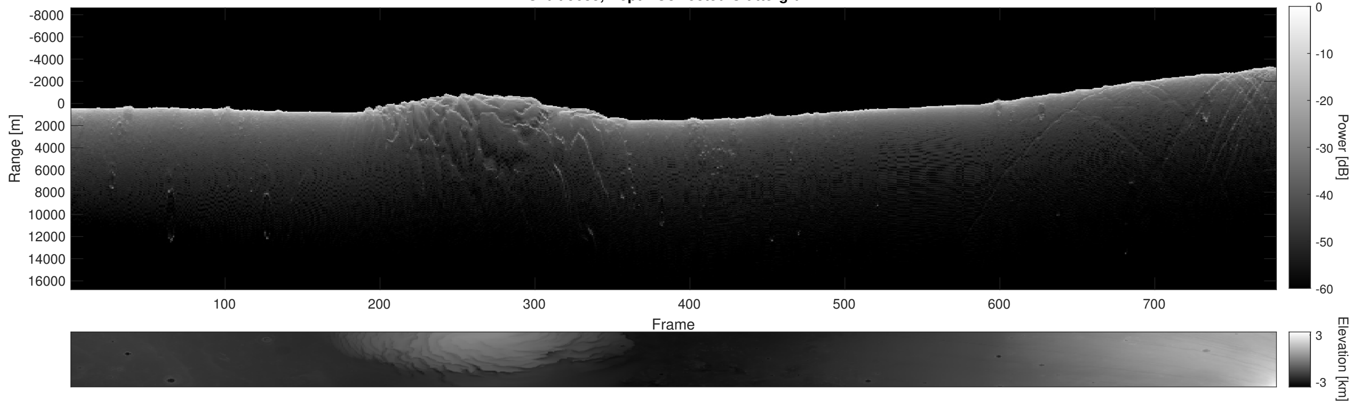
Orbit 9633, Depth-Corrected Cluttergram
