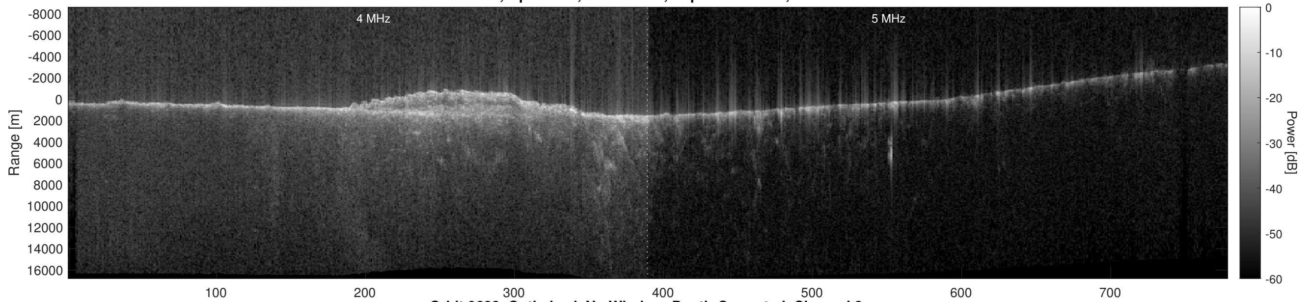
Orbit 9633, Optimized, No Window, Depth-Corrected, Channel 2
