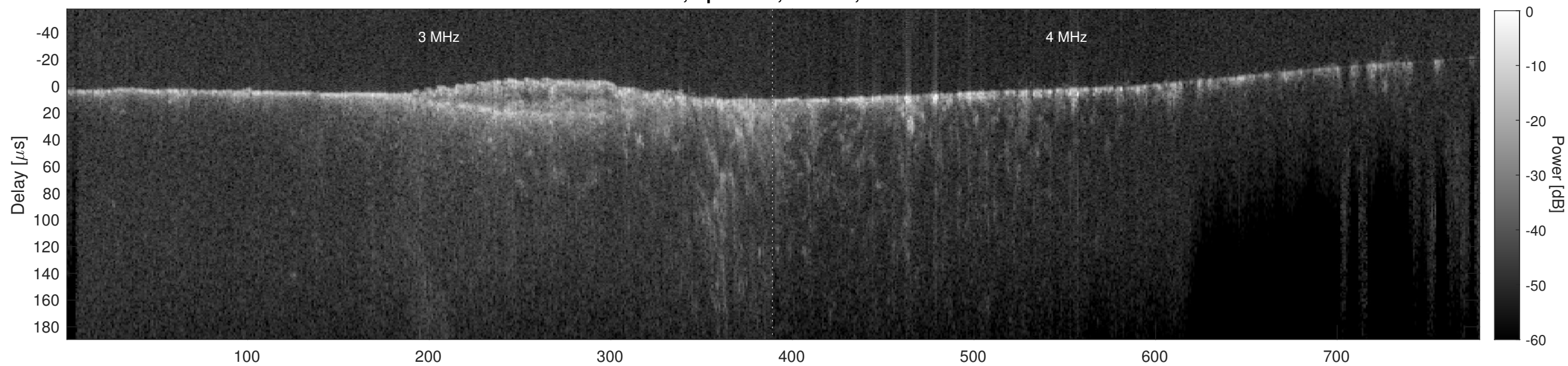
Orbit 9633, Cluttergram
