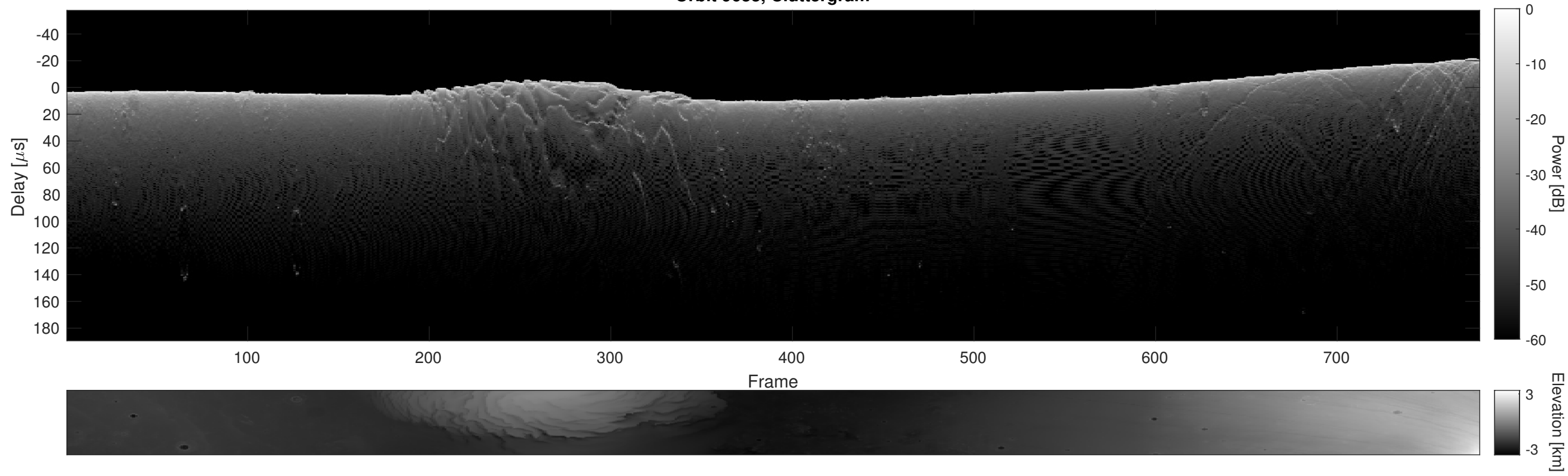
Orbit 9633, Cluttergram
