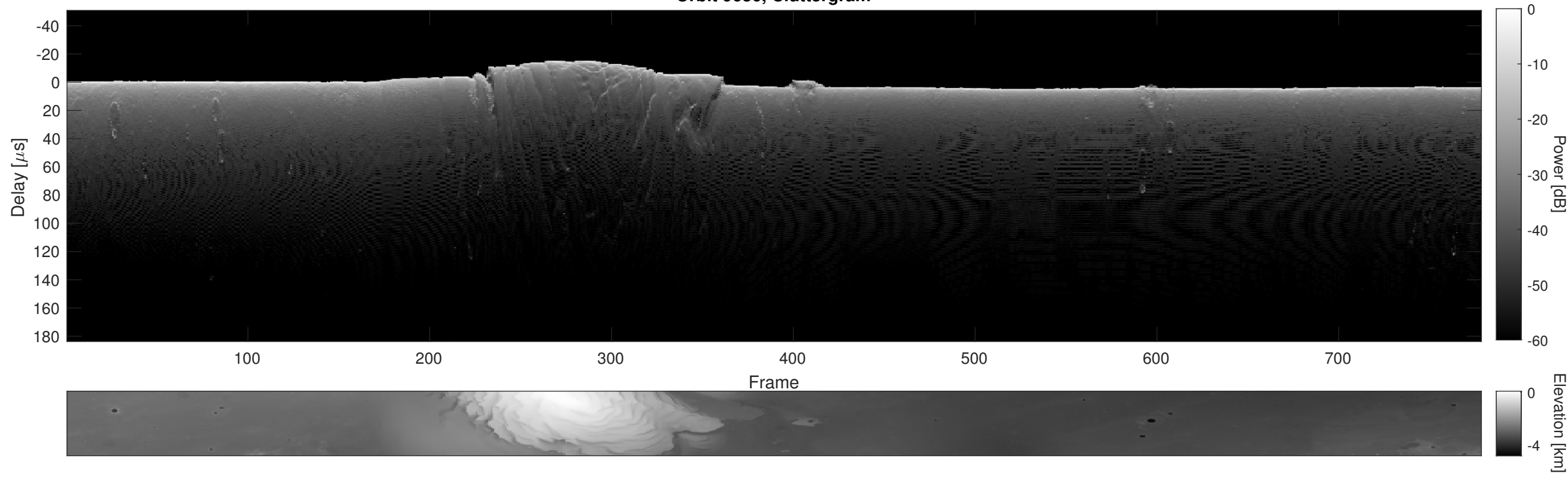
Orbit 9636, Cluttergram
