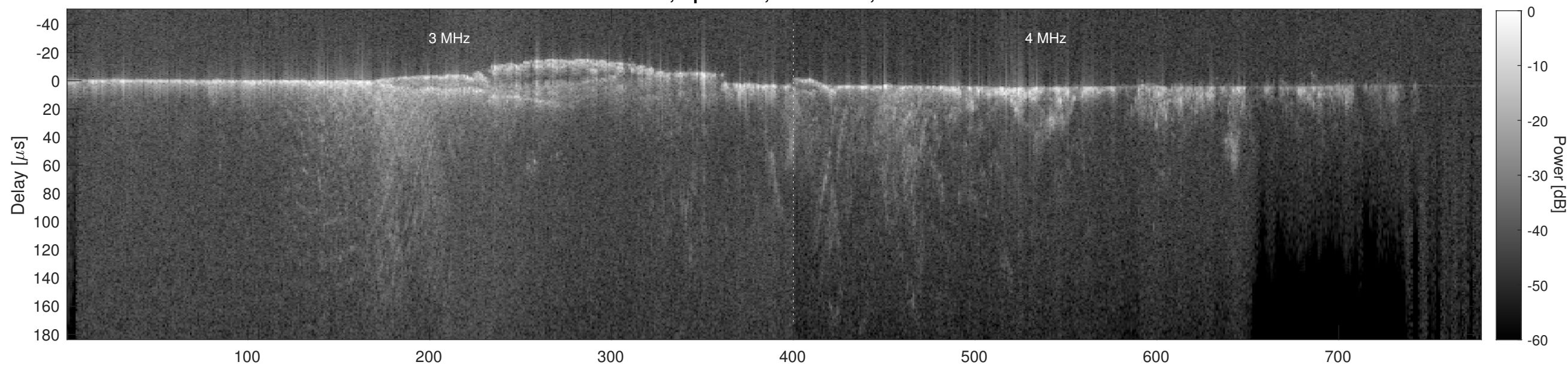
Orbit 9636, Cluttergram
