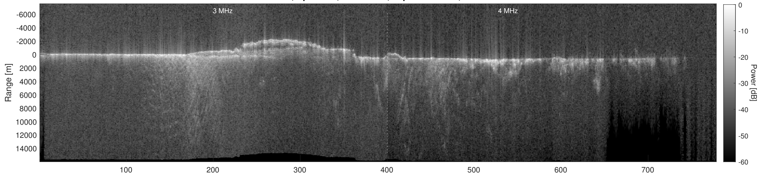
Orbit 9636, Depth-Corrected Cluttergram
