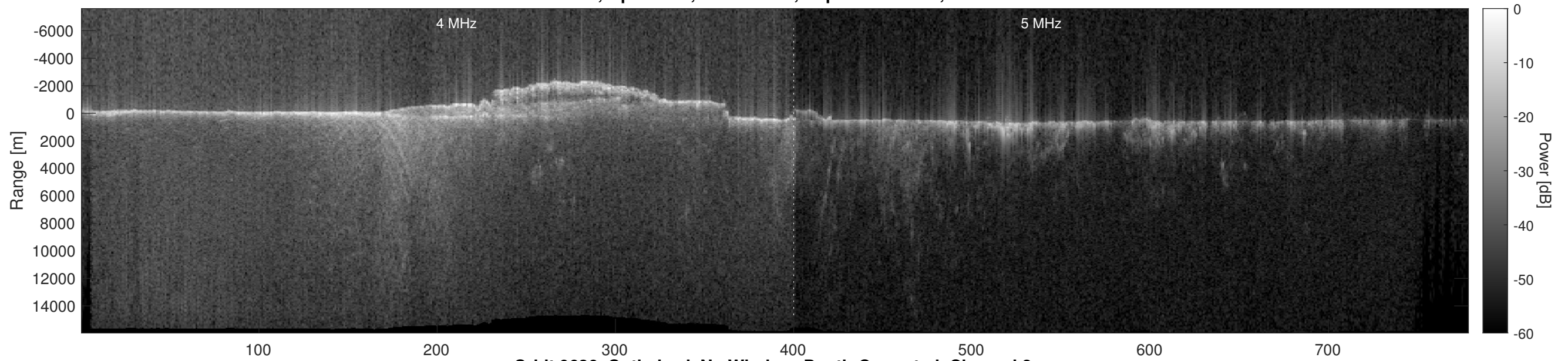
Orbit 9636, Optimized, No Window, Depth-Corrected, Channel 2
