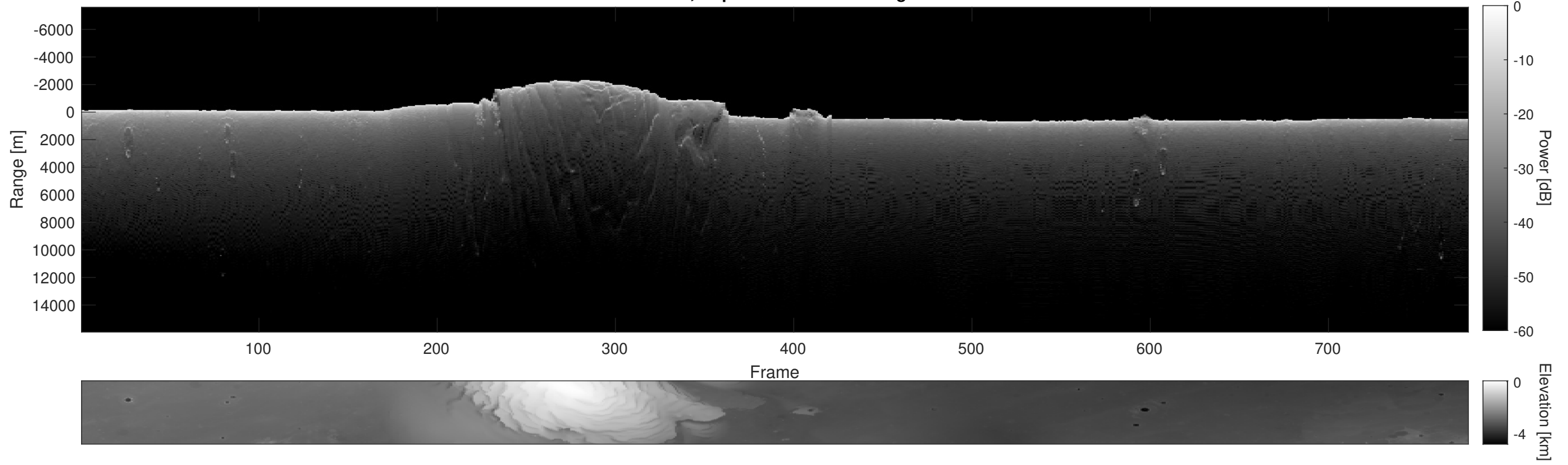
Orbit 9636, Depth-Corrected Cluttergram
