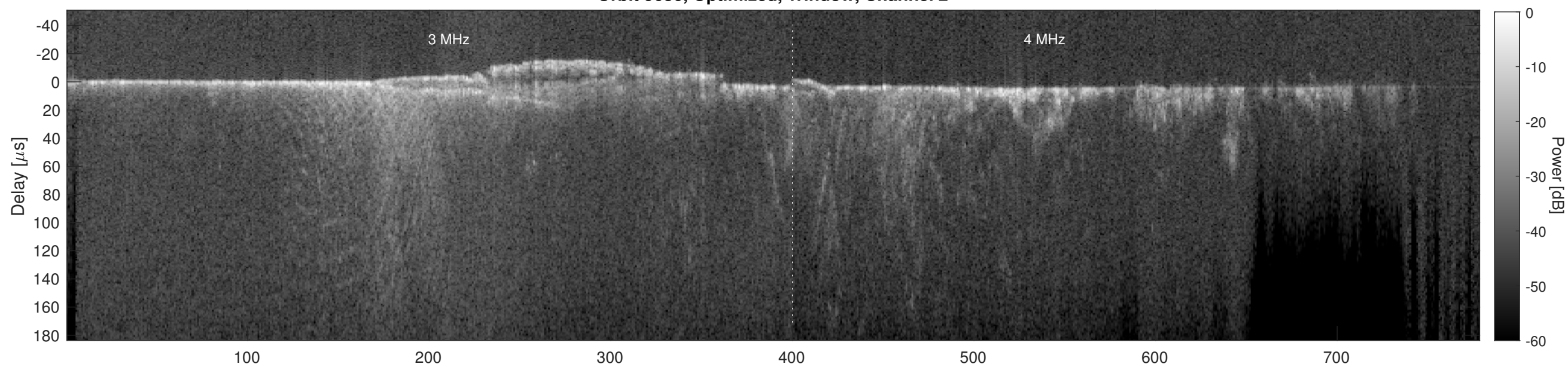
Orbit 9636, Cluttergram
