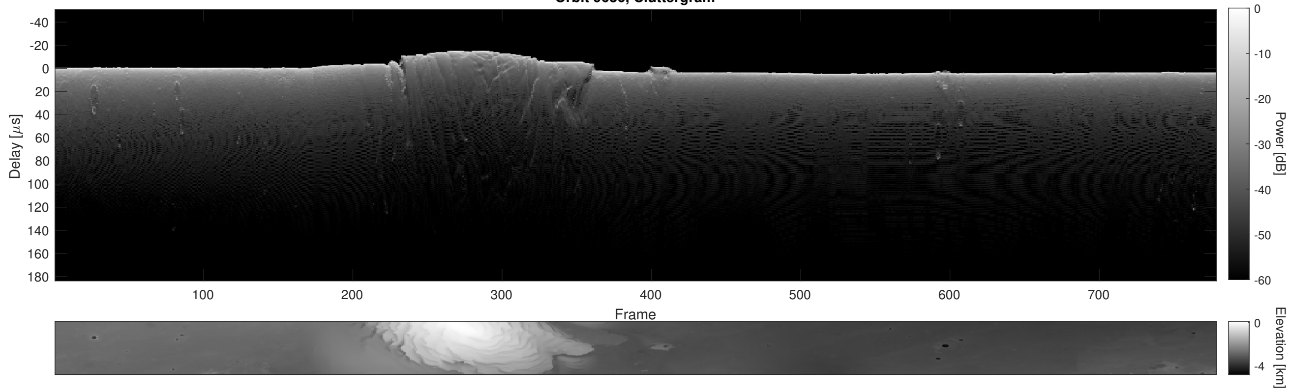
Orbit 9636, Cluttergram
