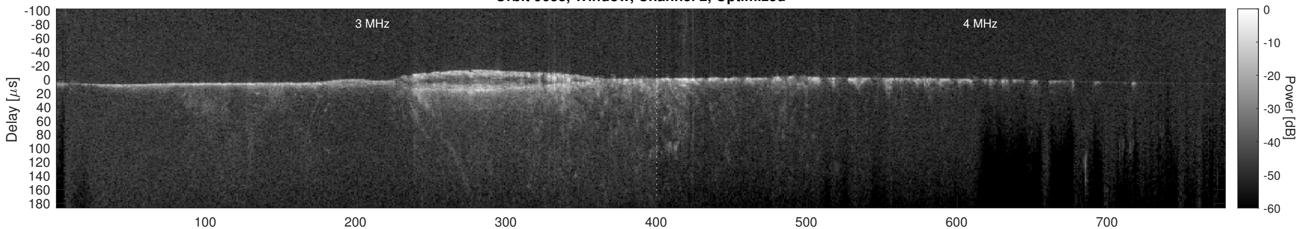
Orbit 9638, Cluttergram
