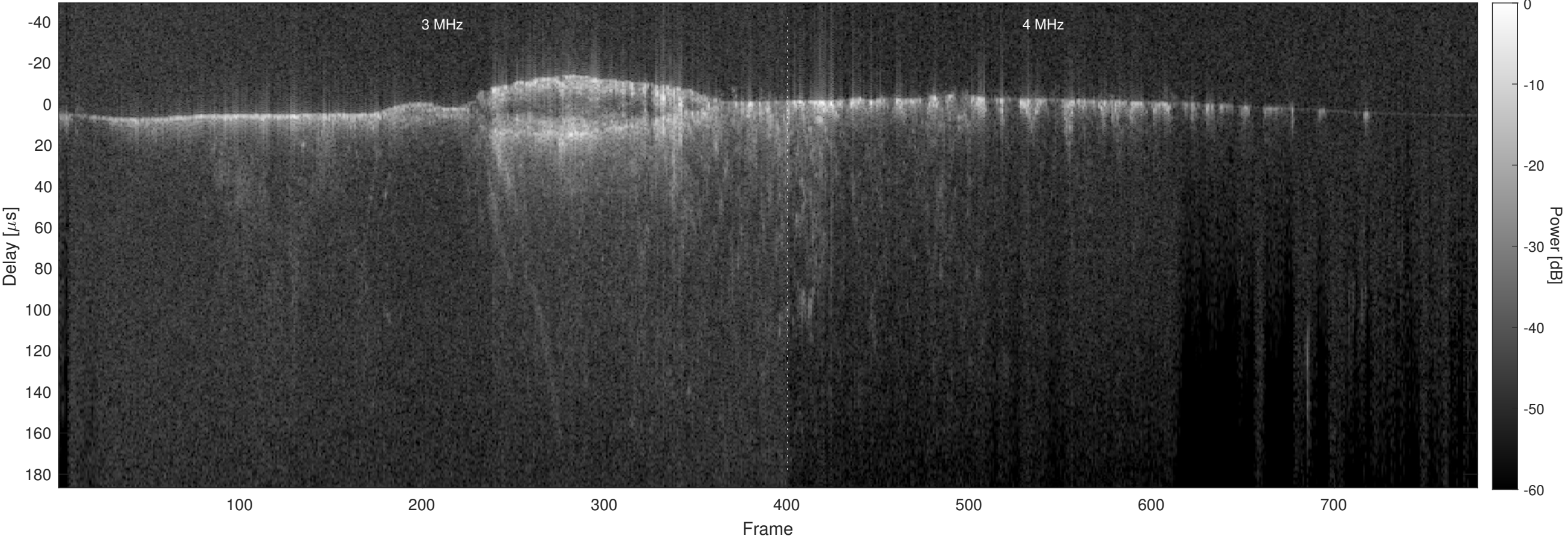
Orbit 9638, Optimized, No Window, Channel 2
