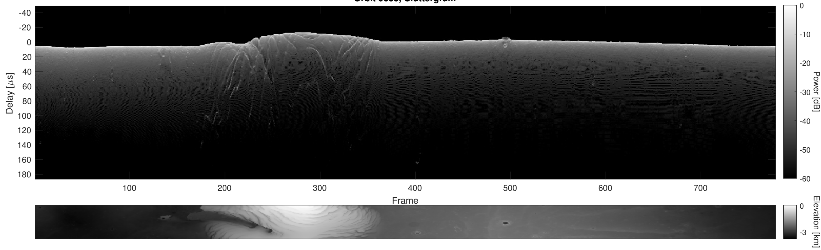
Orbit 9638, Cluttergram
